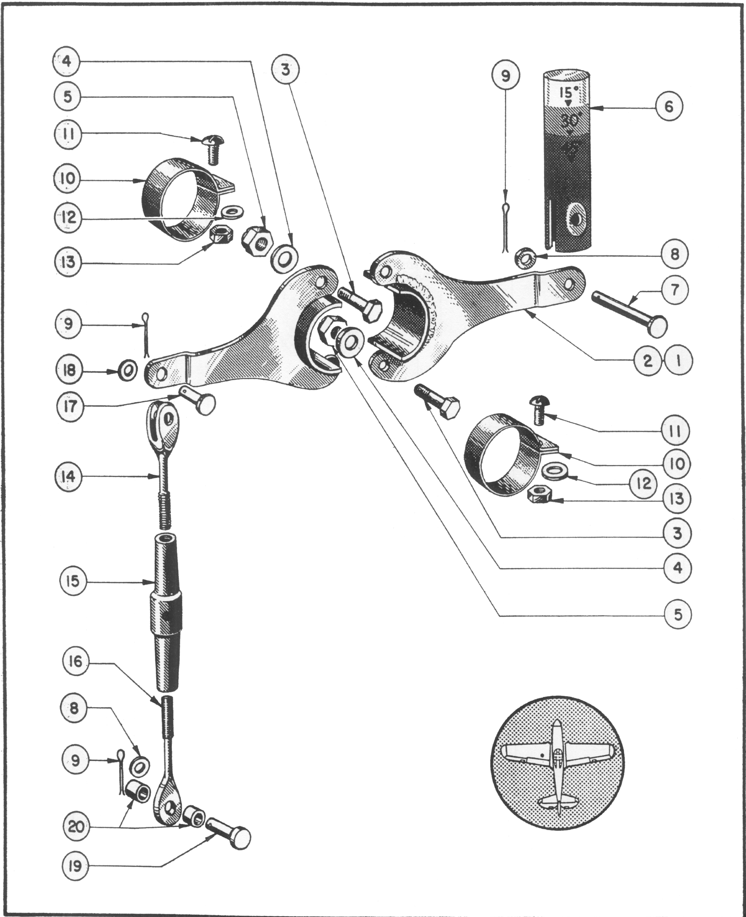
Figure 10—Flap Position Indicator
