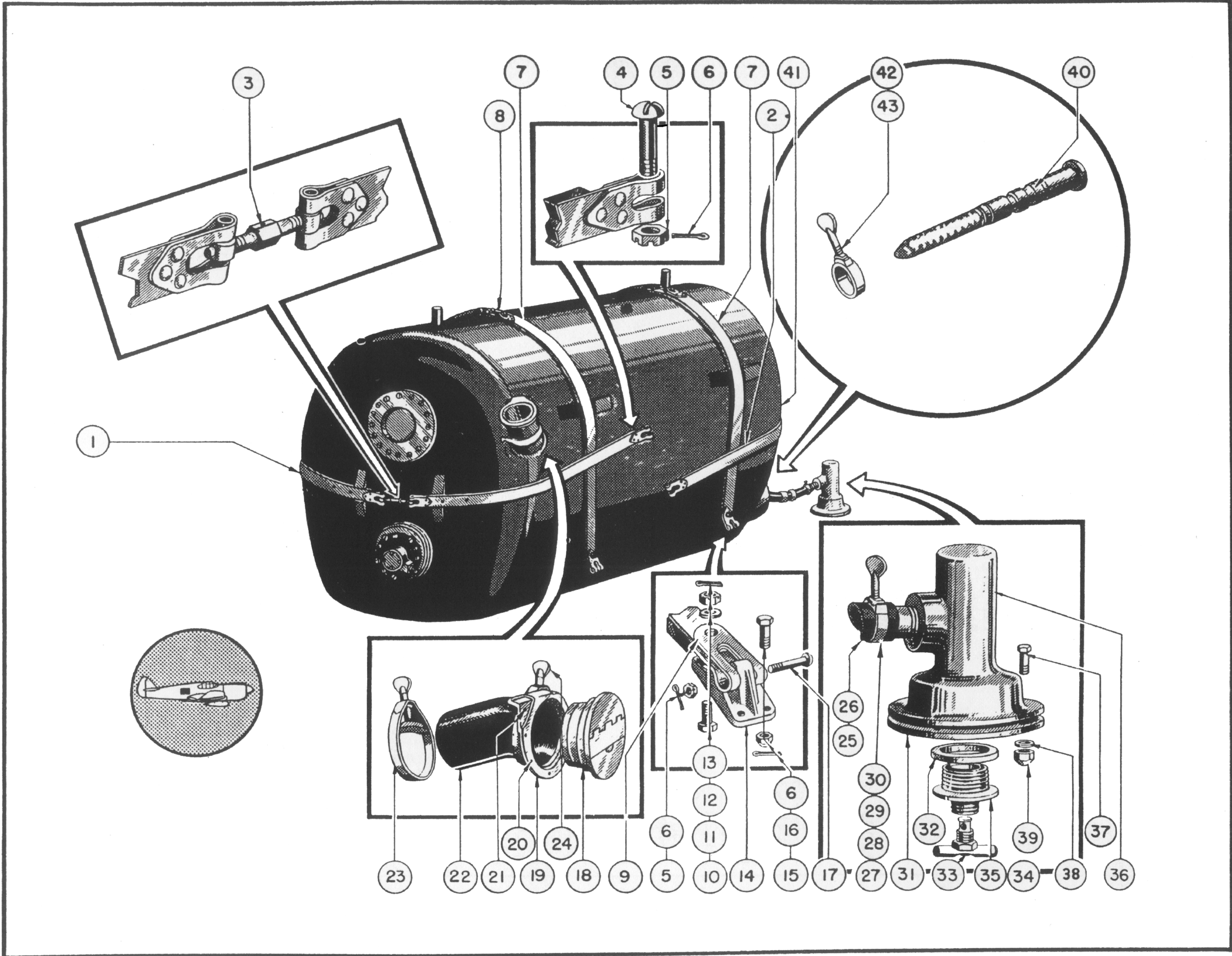
Figure 101—Fuselage Fuel Tank
