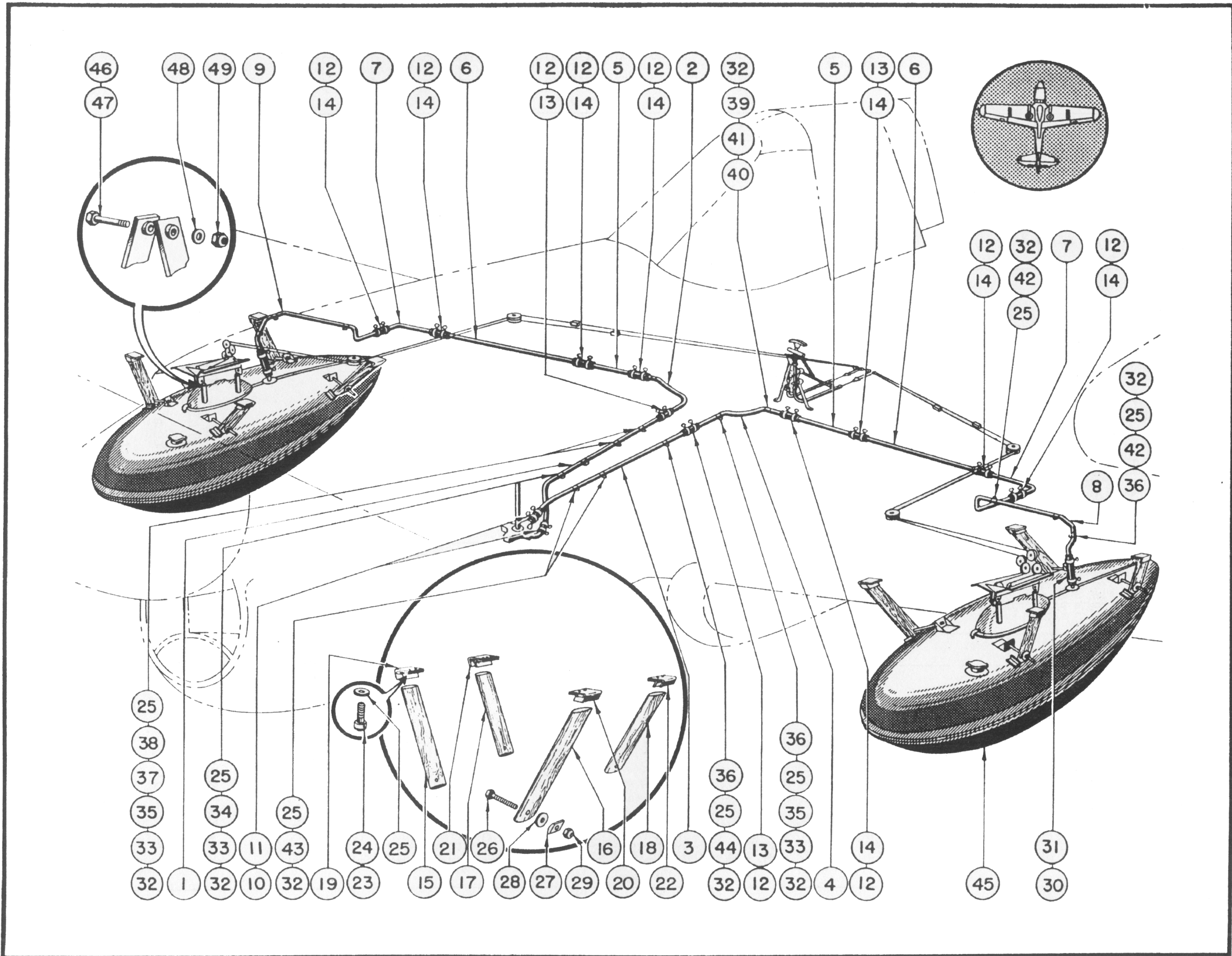
Figure 102—Auxiliary Wing Tank Fuel System Installation
