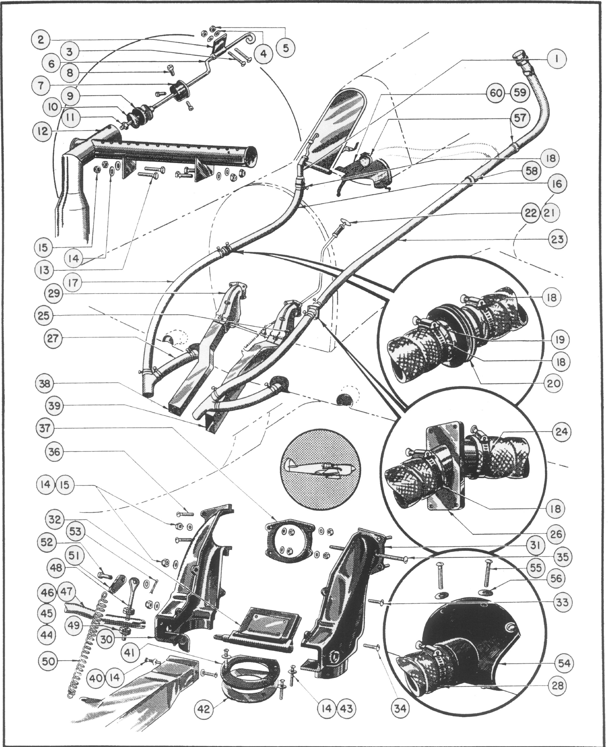
Figure 103—Heat and Vent System Installation
