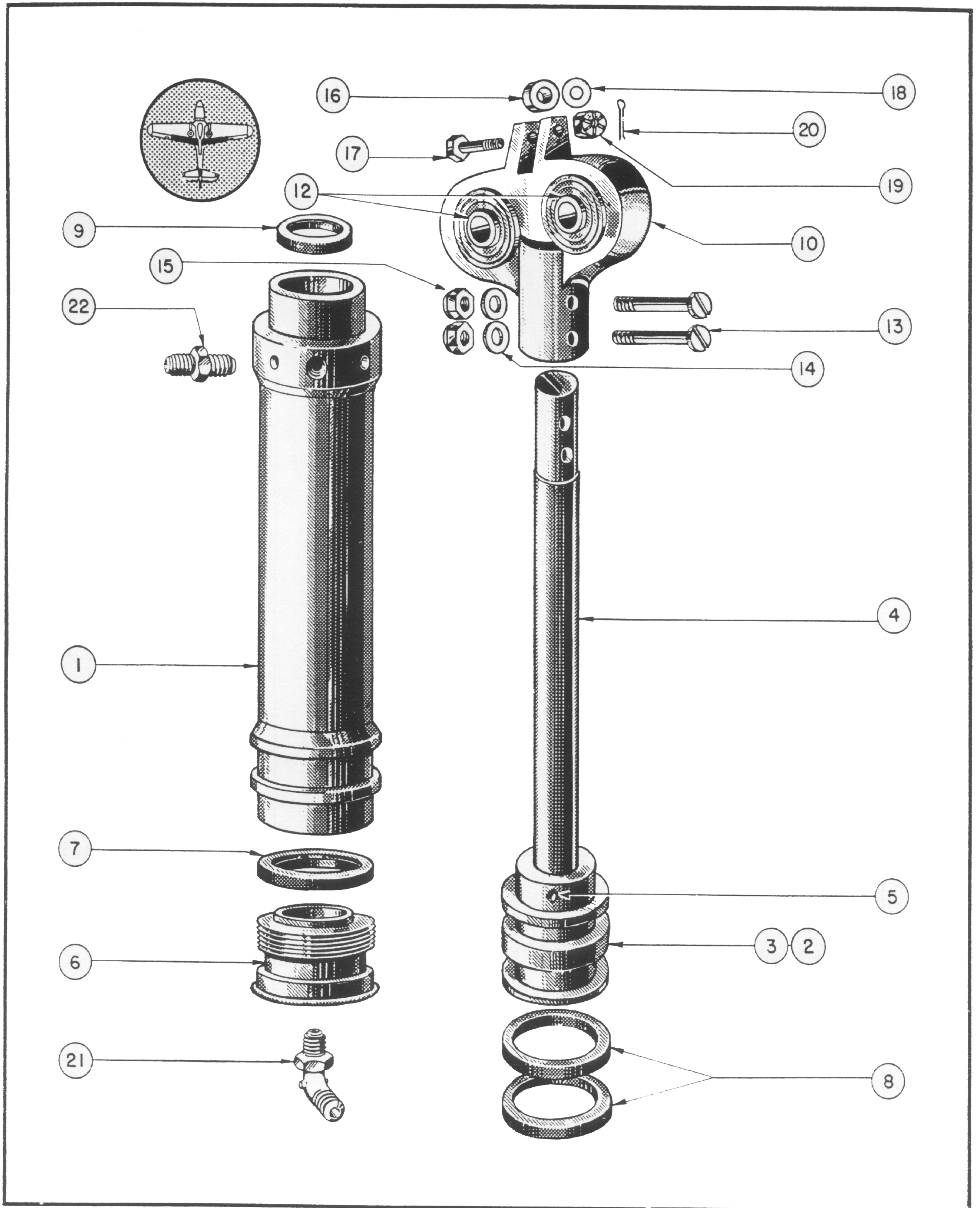
Figure 104—Flap Actuating Cylinder Assembly
