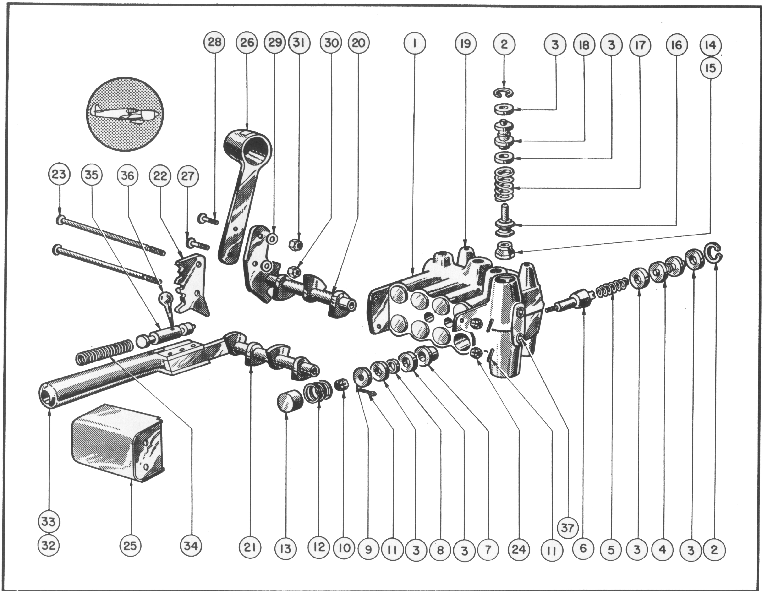
Figure 106—Poppet Valve Assembly
