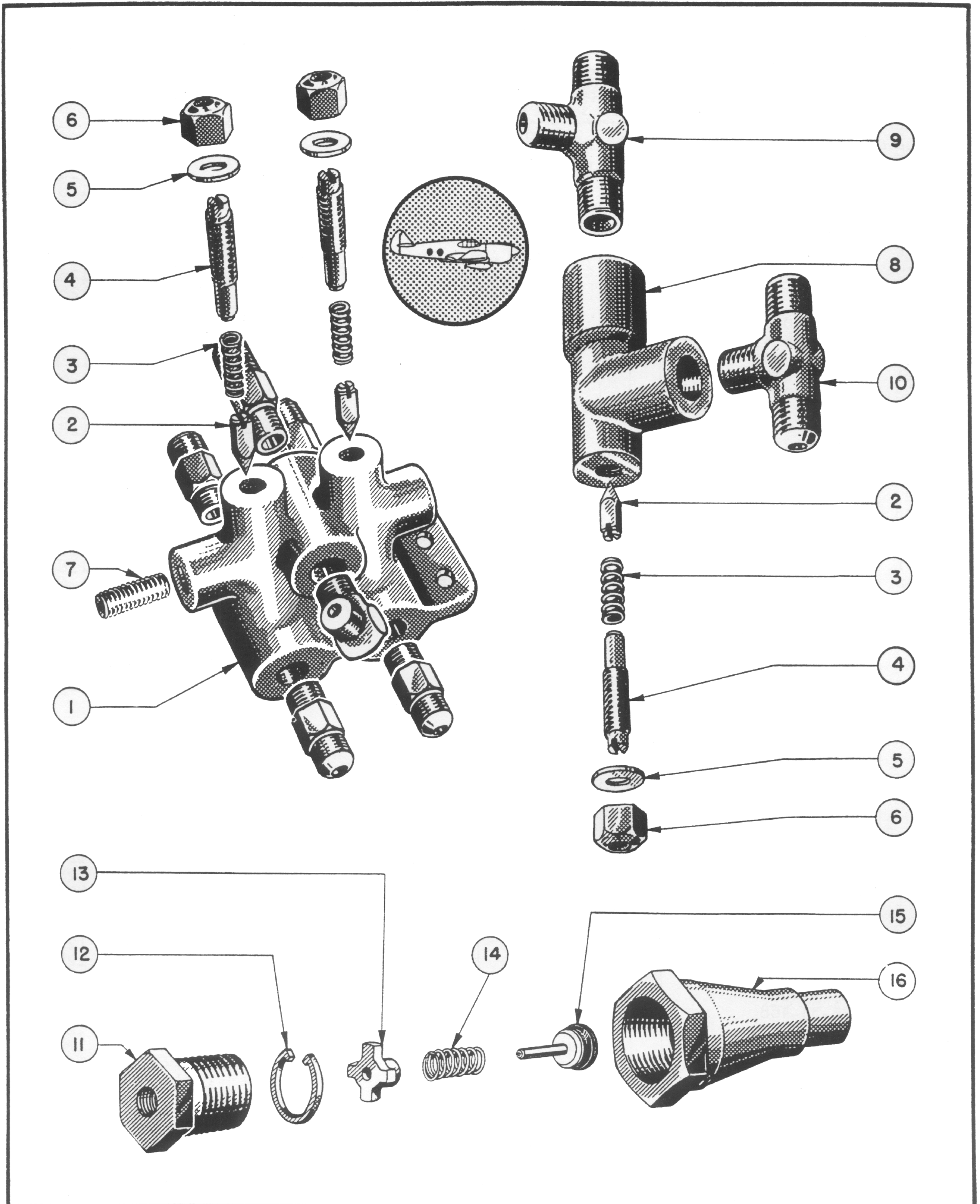
Figure 107—Relief and Check Valves
