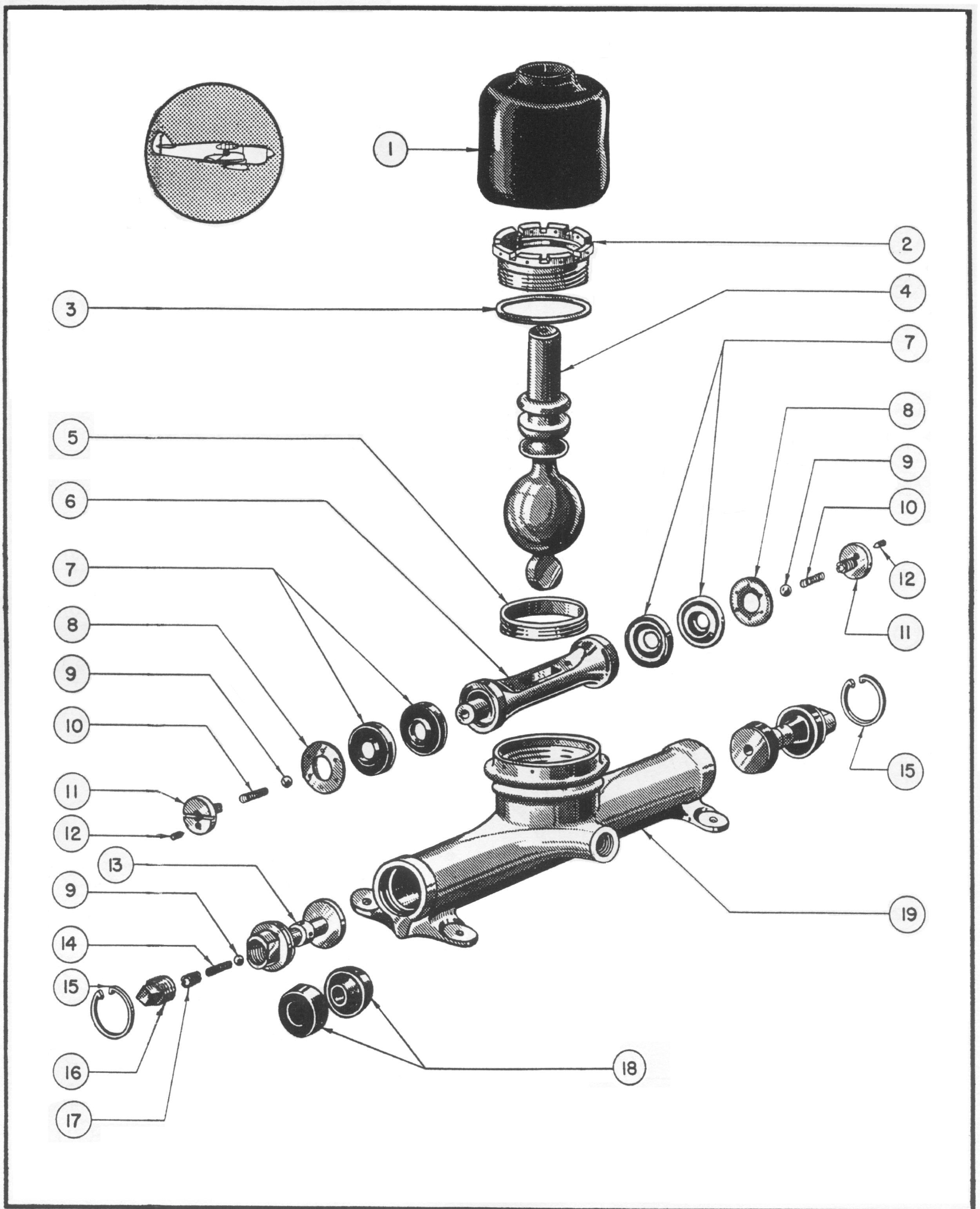
Figure 108—Hand Pump Assembly
