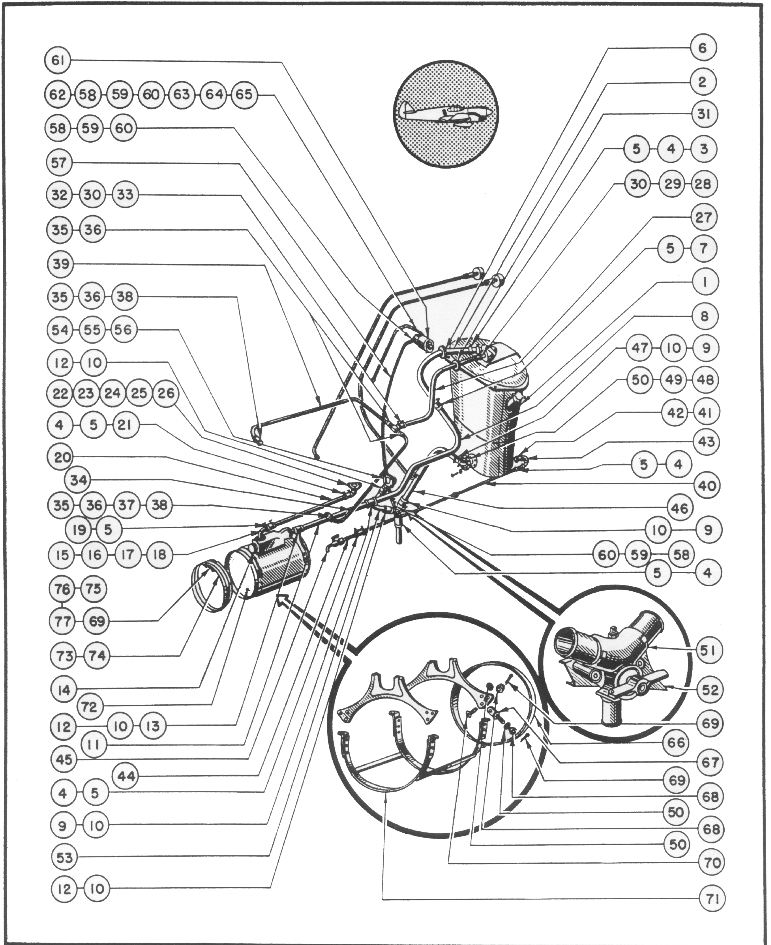
Figure 109—Oil System Installation (A-B)
