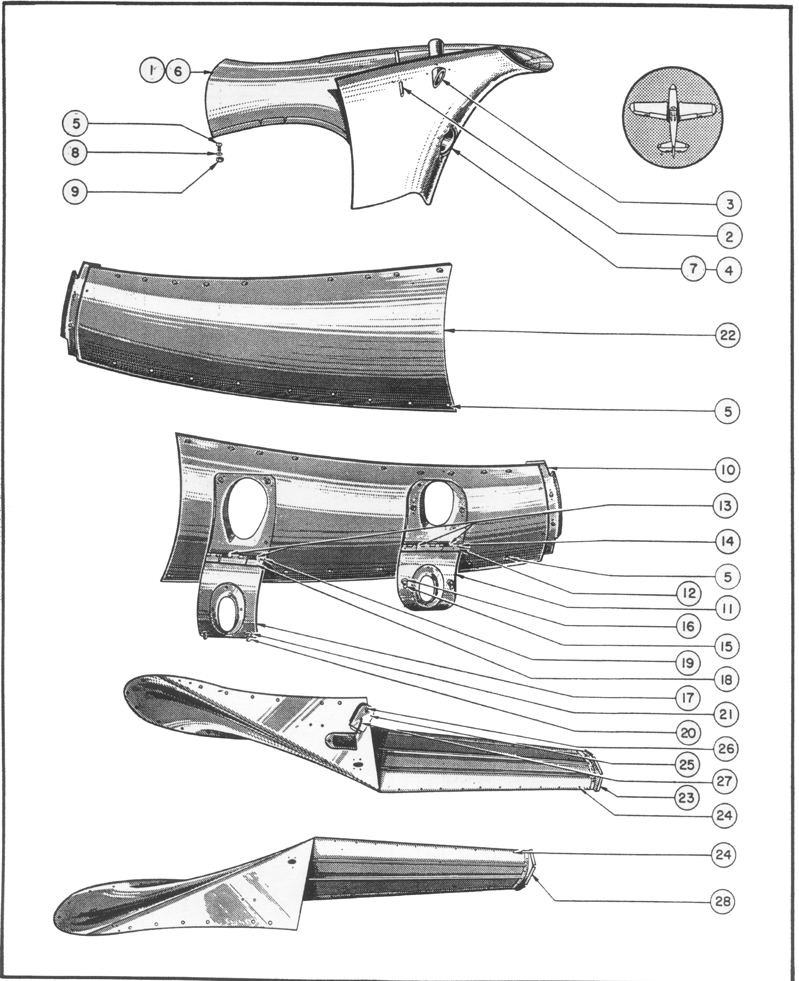
Figure 11—Wing Fillets
