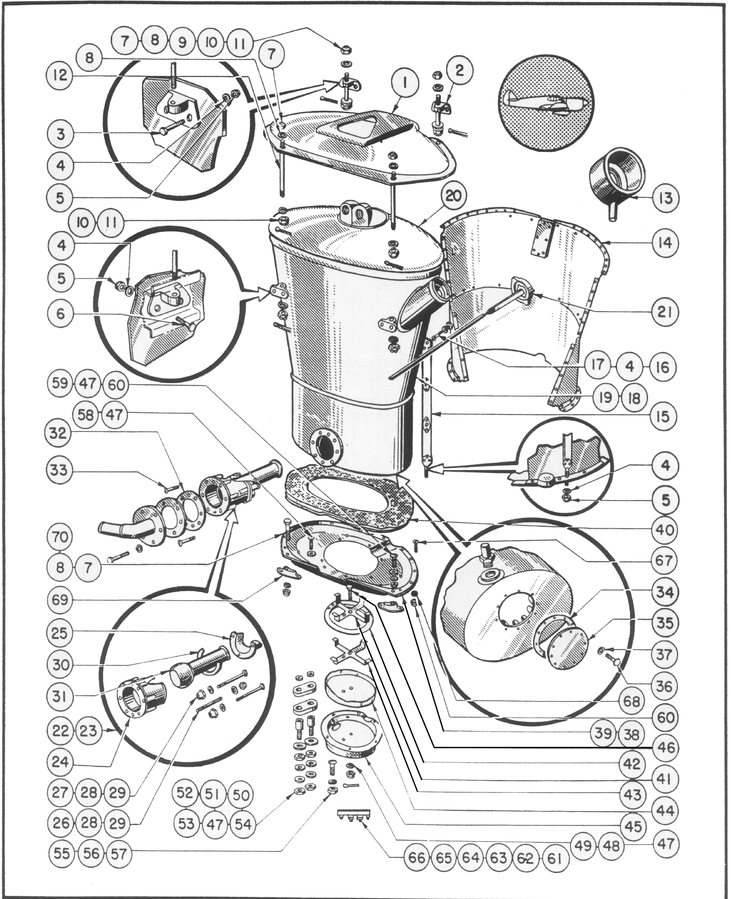
Figure 110—Oil Tank Installation (A-B)
