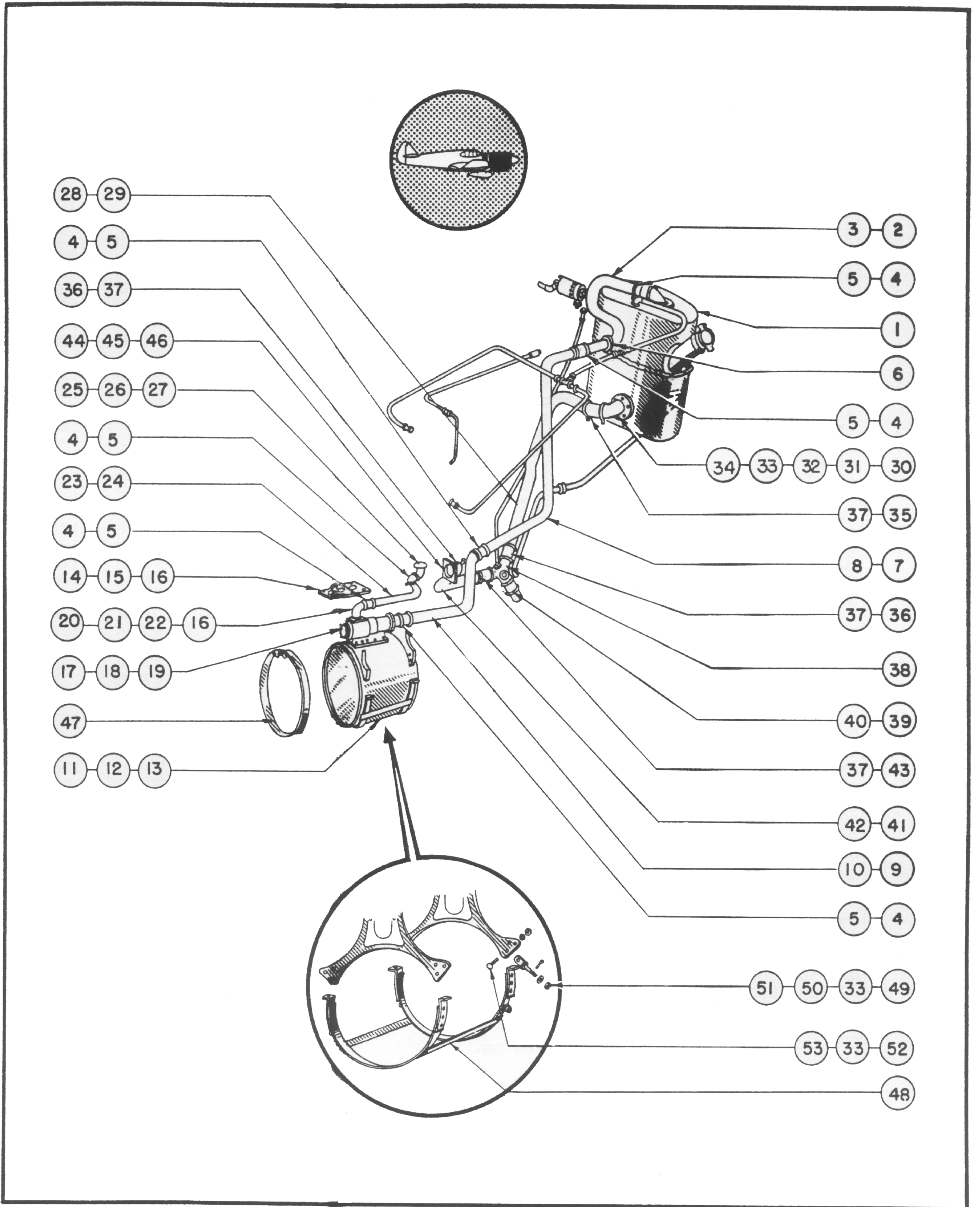
Figure 111—Oil System Installation (C-T)
