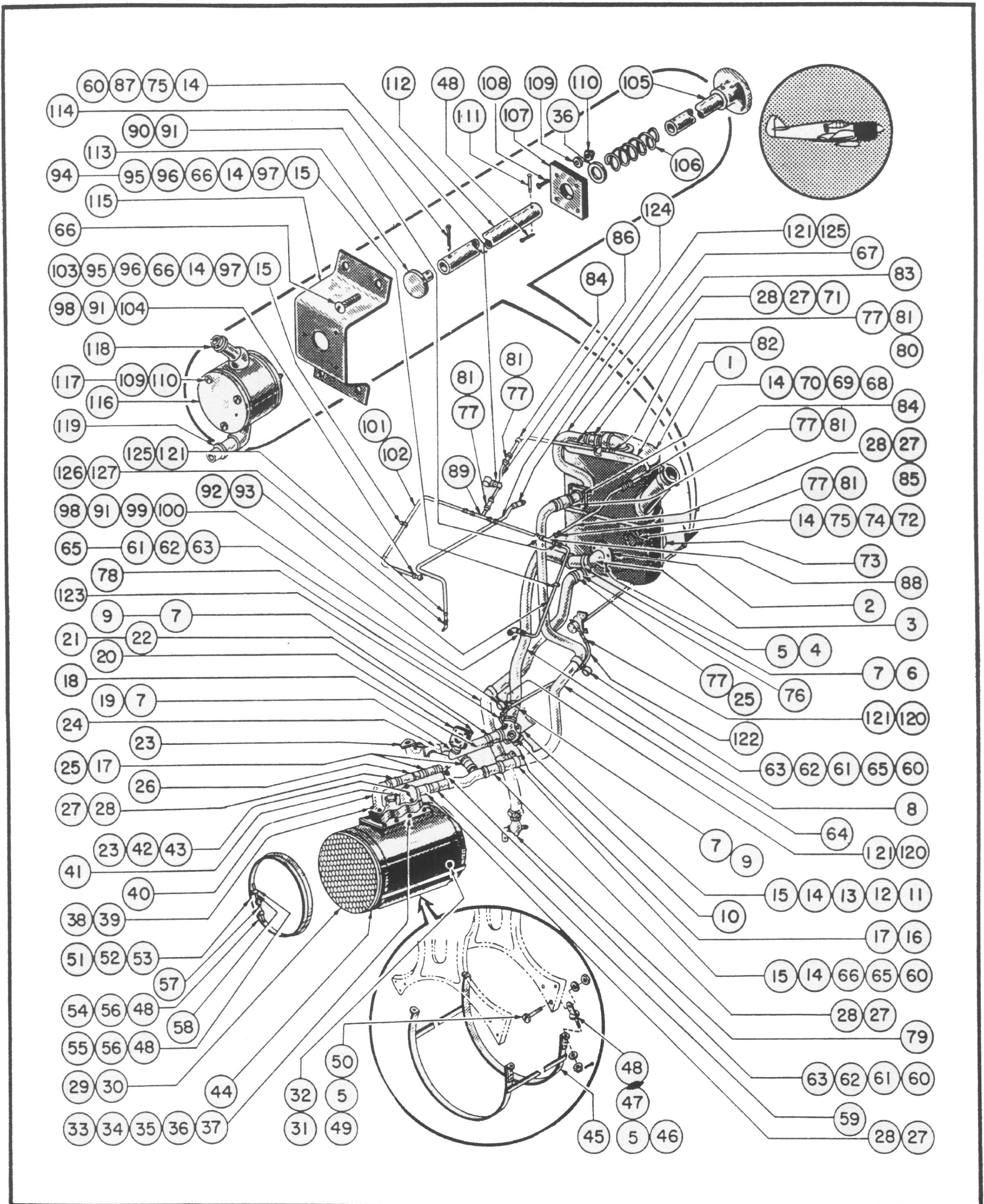
Figure 112—Oil System Installation (U-W)
