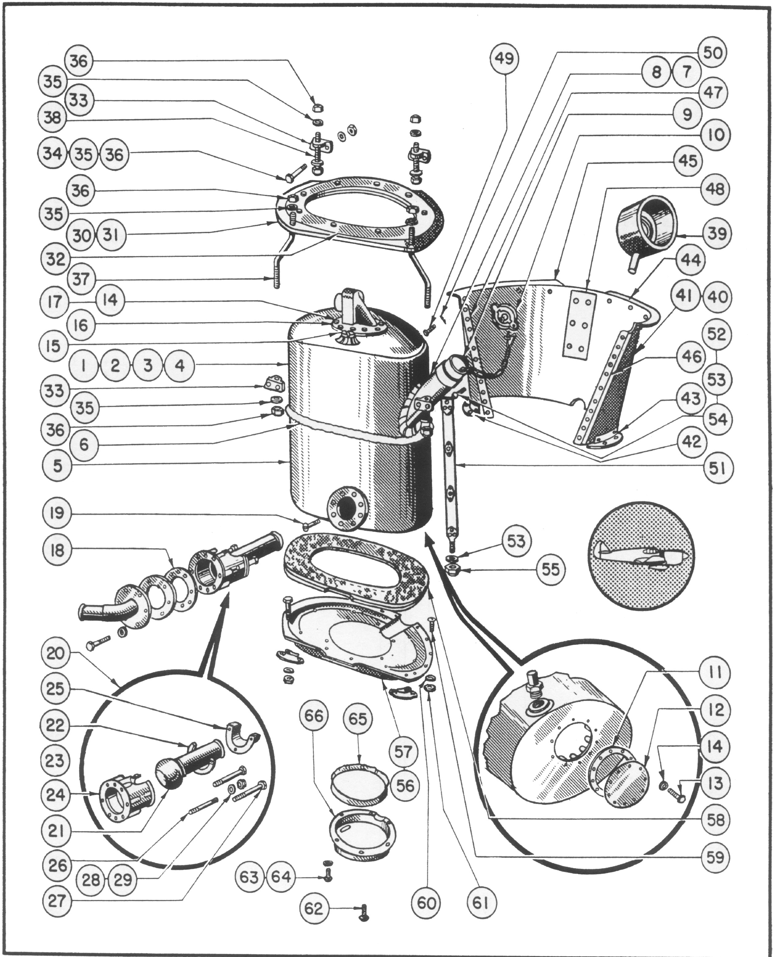
Figure 113—Oil Tank Installation (C-W)
