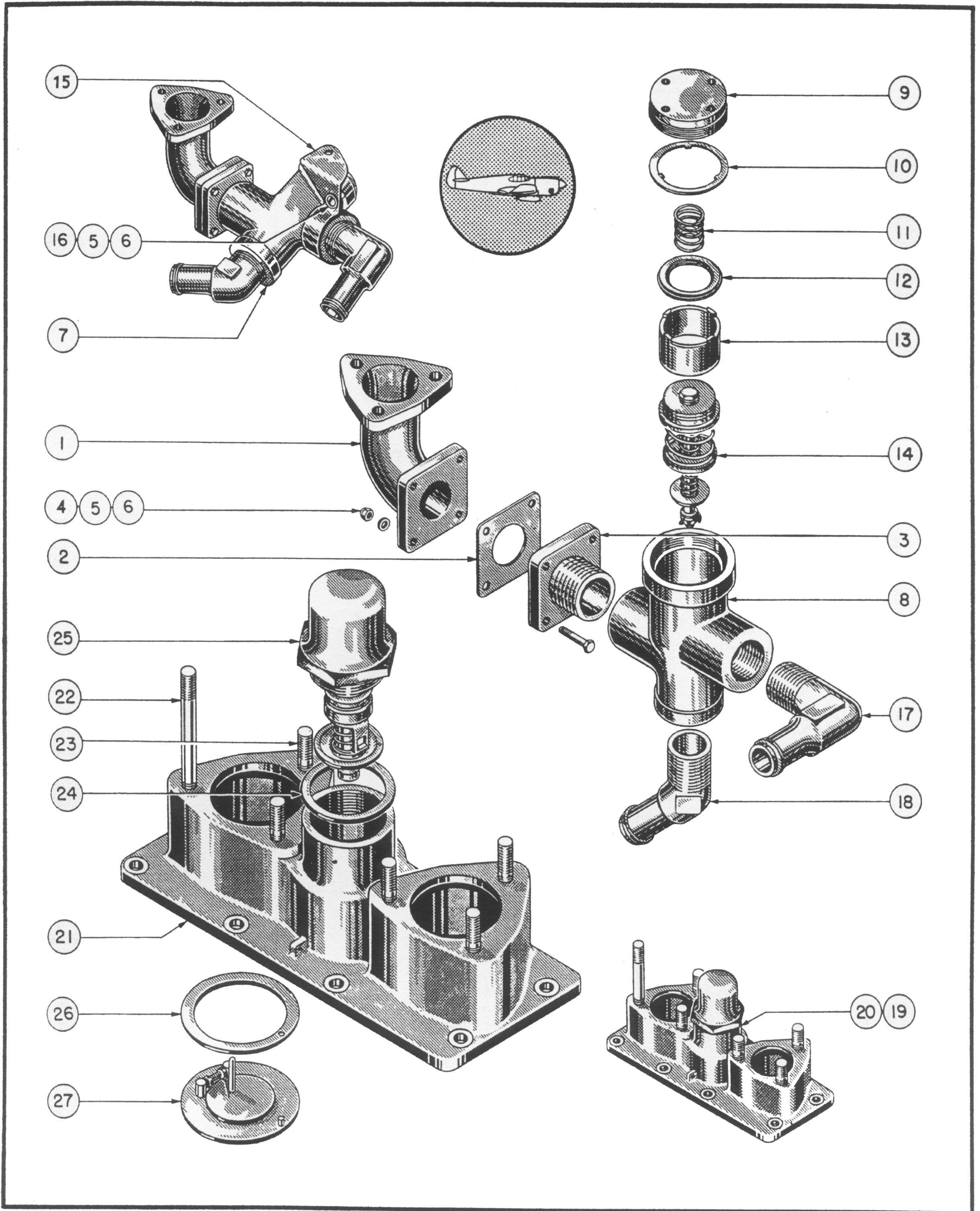
Figure 114—Scavenger Pump Outlet & Oil Temperature Regulator Valve Assemblies
