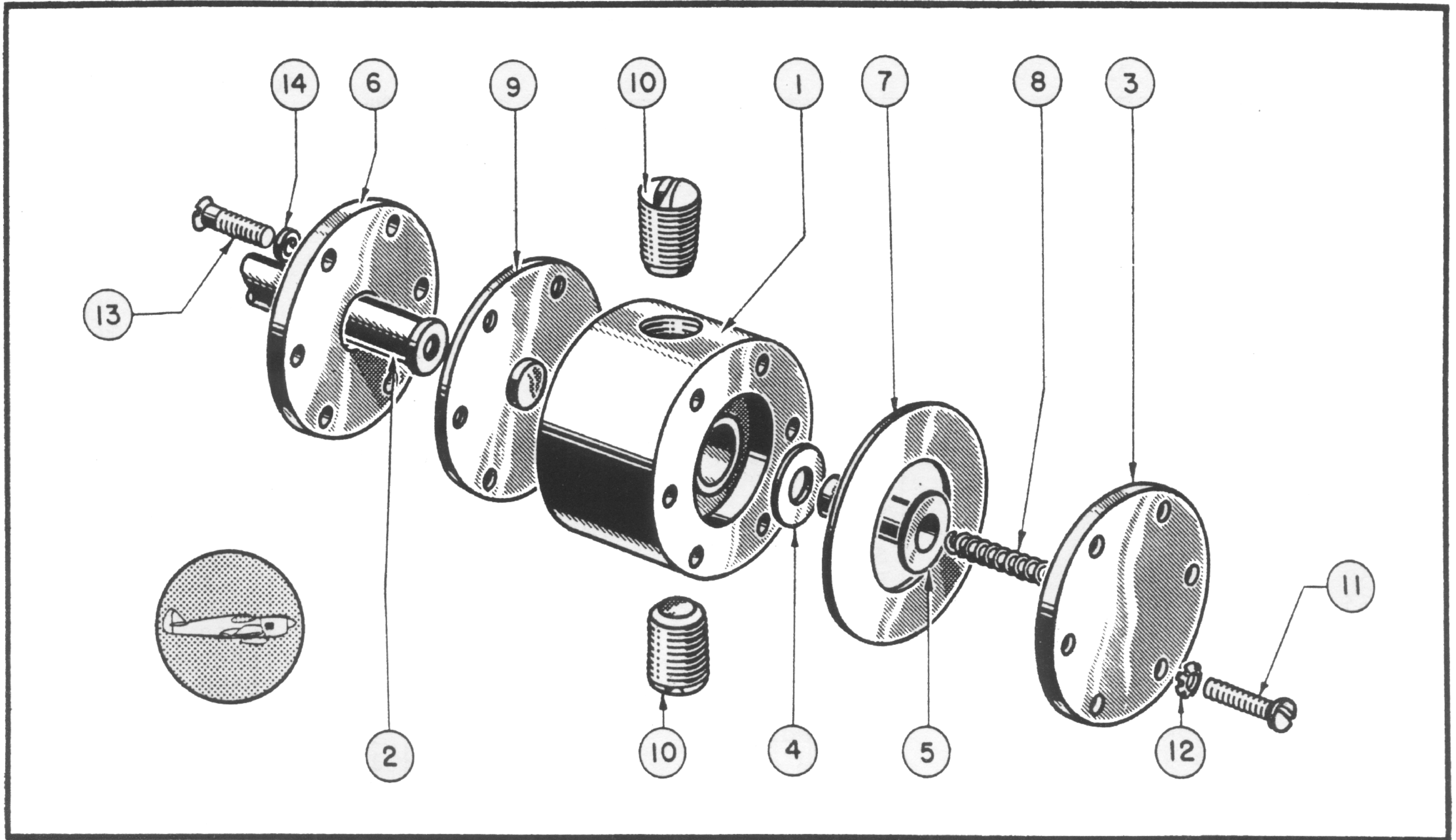
Figure 115—Oil Dilution Valve
