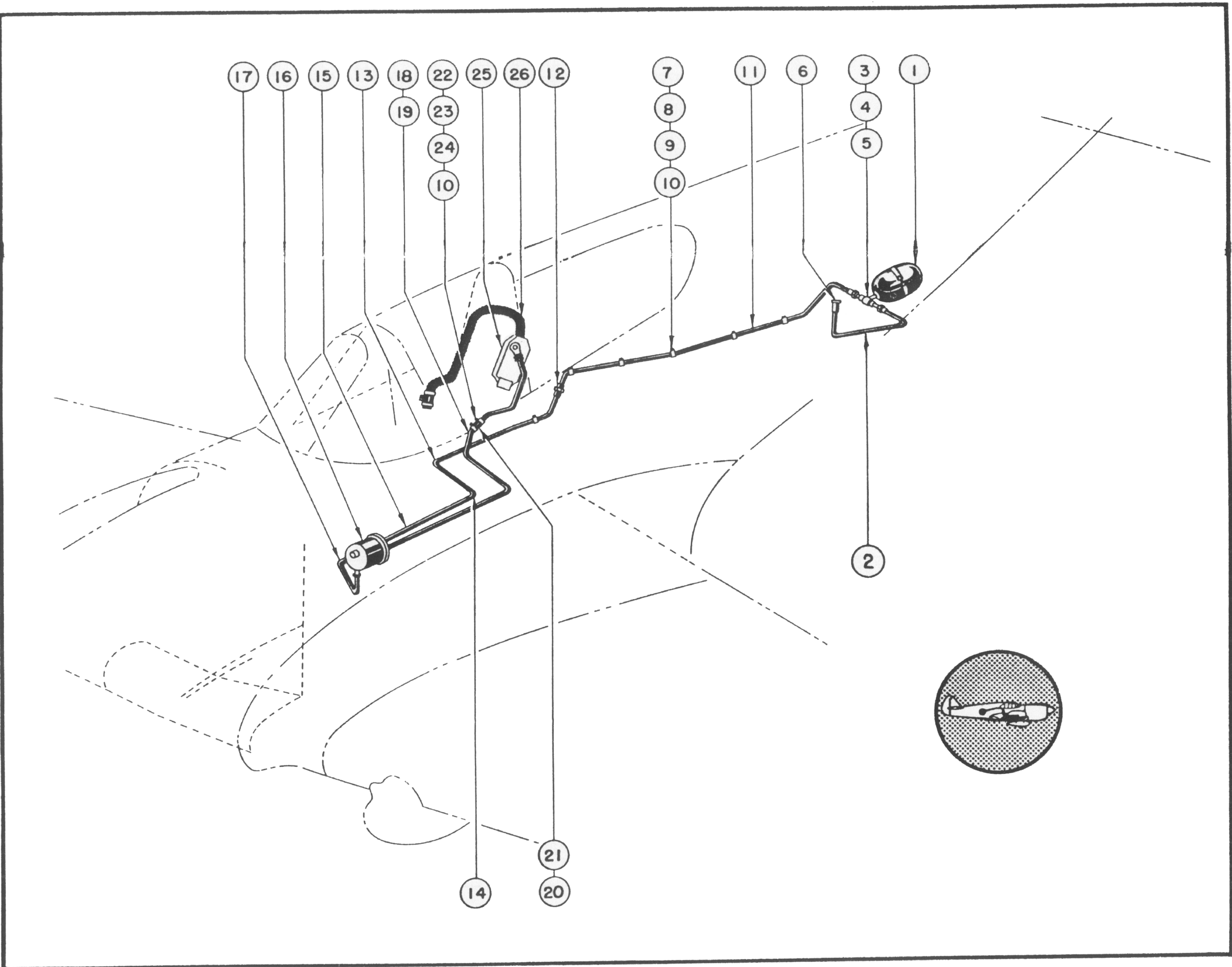
Figure 116—Oxygen System Installation (A-AF43-5477)
