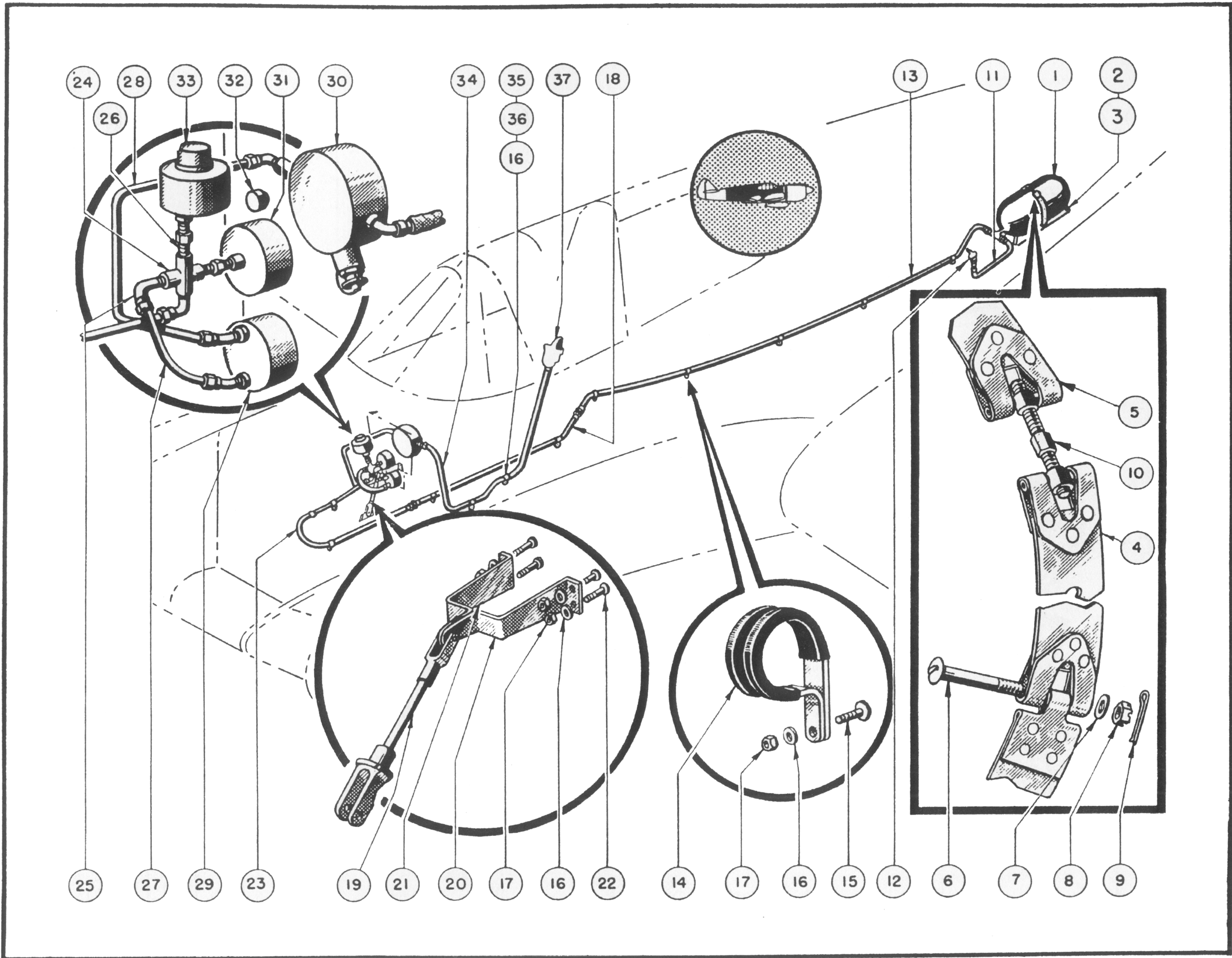
Figure 117—Oxygen System Installation (AF43-5478—B)
