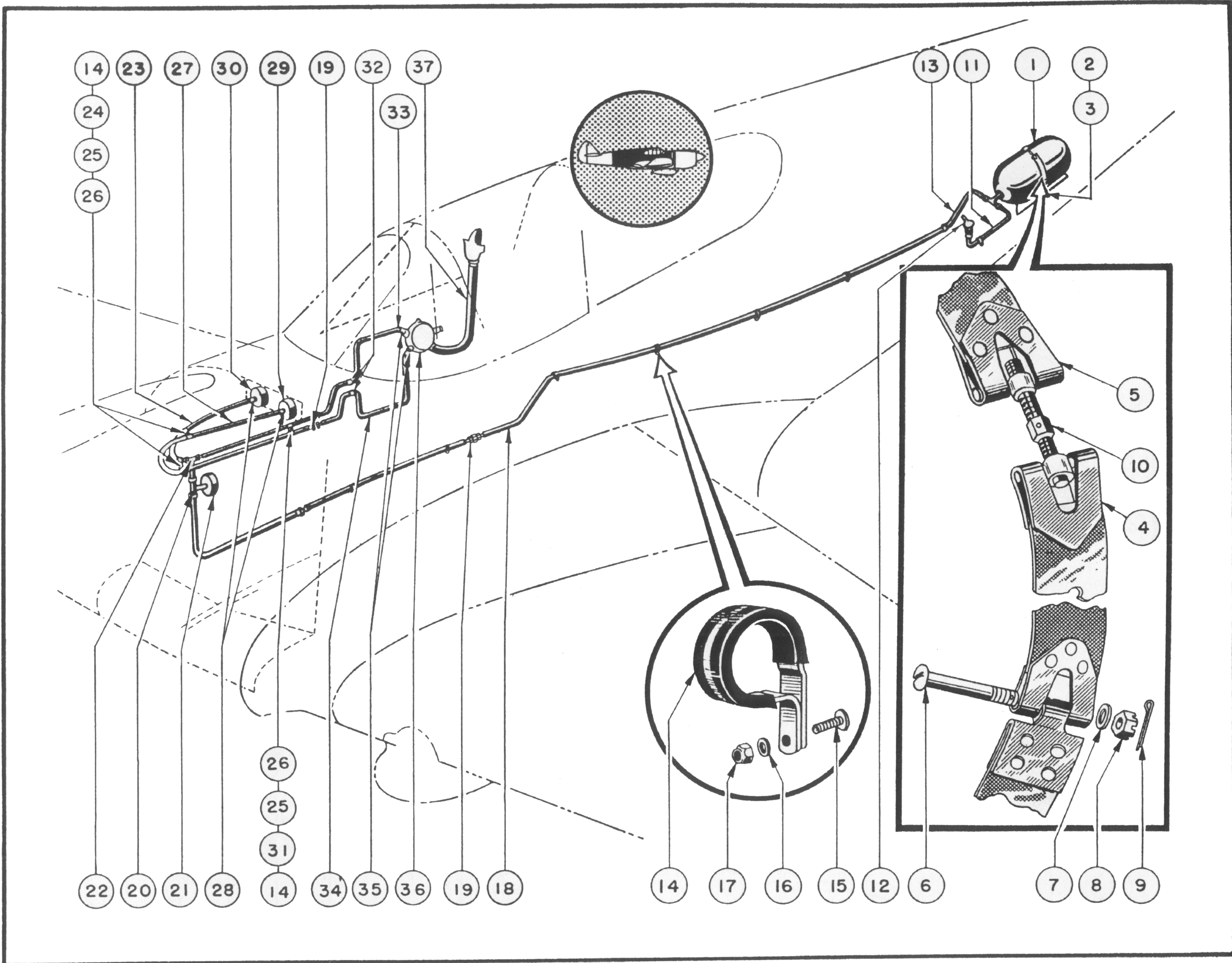
Figure 118—Oxygen System Installation (C-D)
