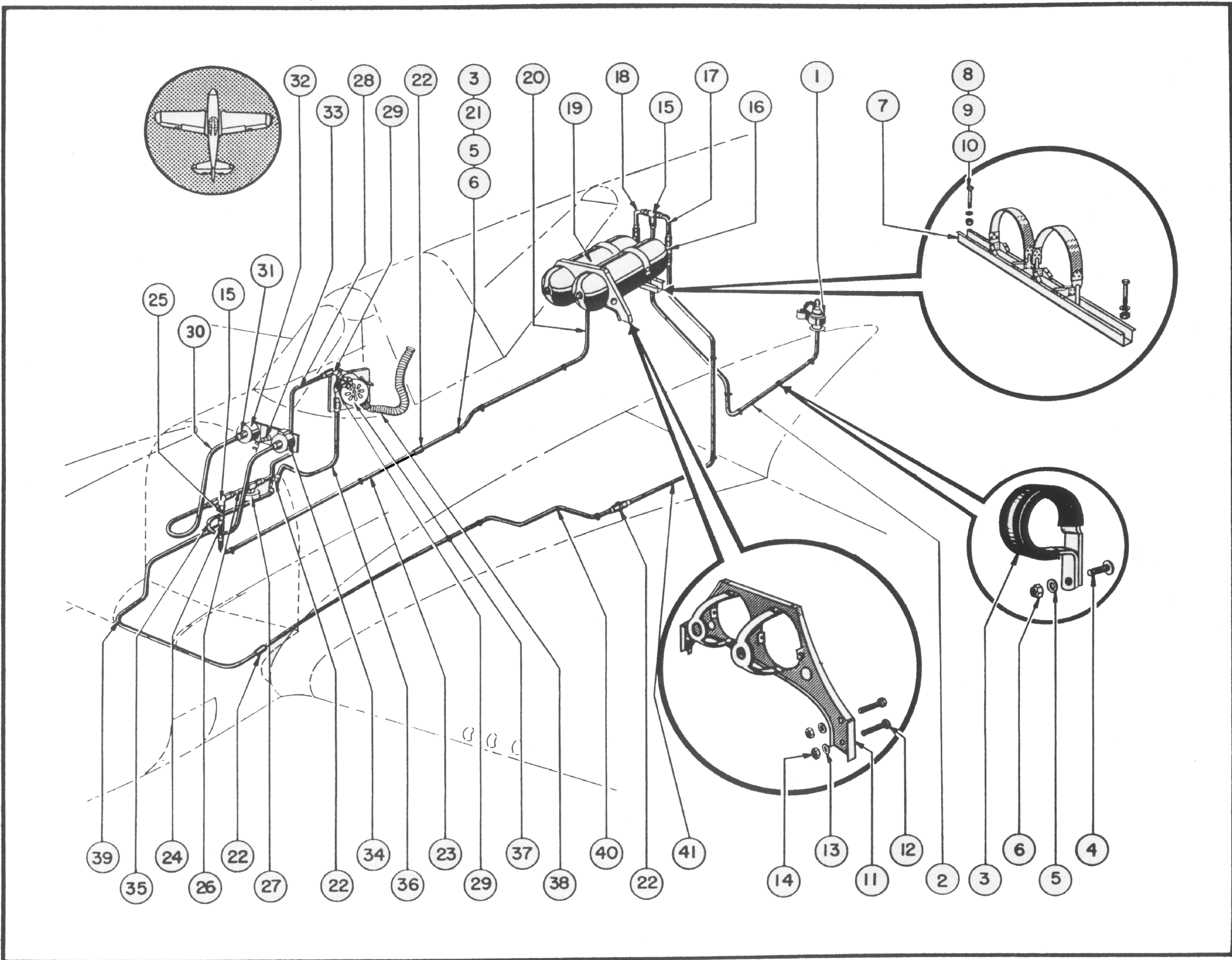
Figure 119—Oxygen System Installation (E-W)
