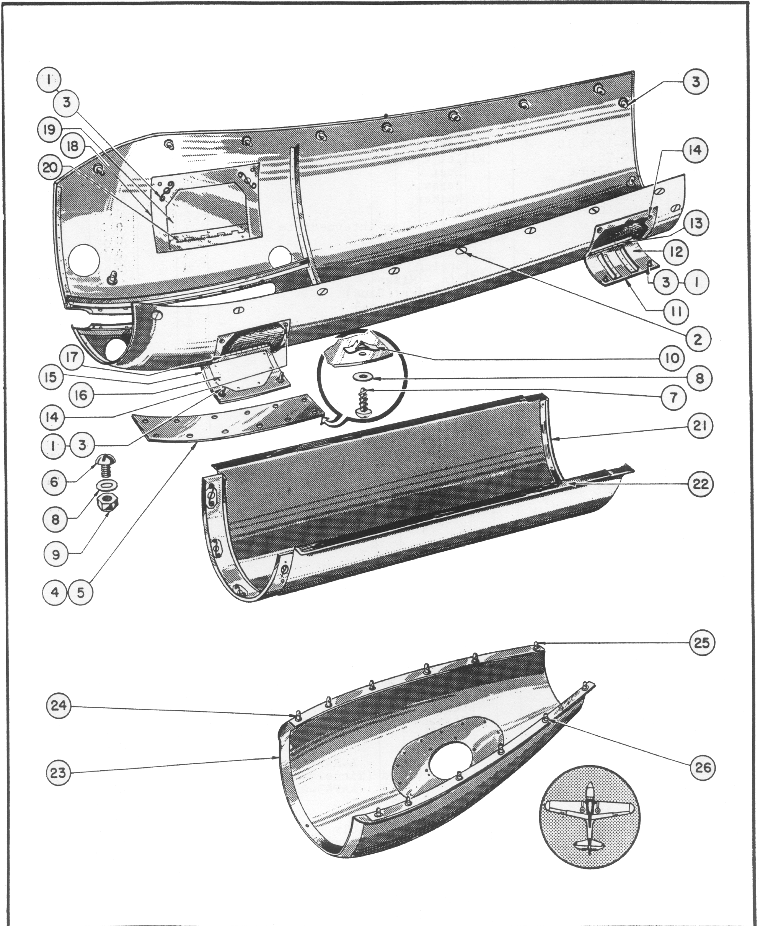
Figure 12—Forward Keel Fairing
