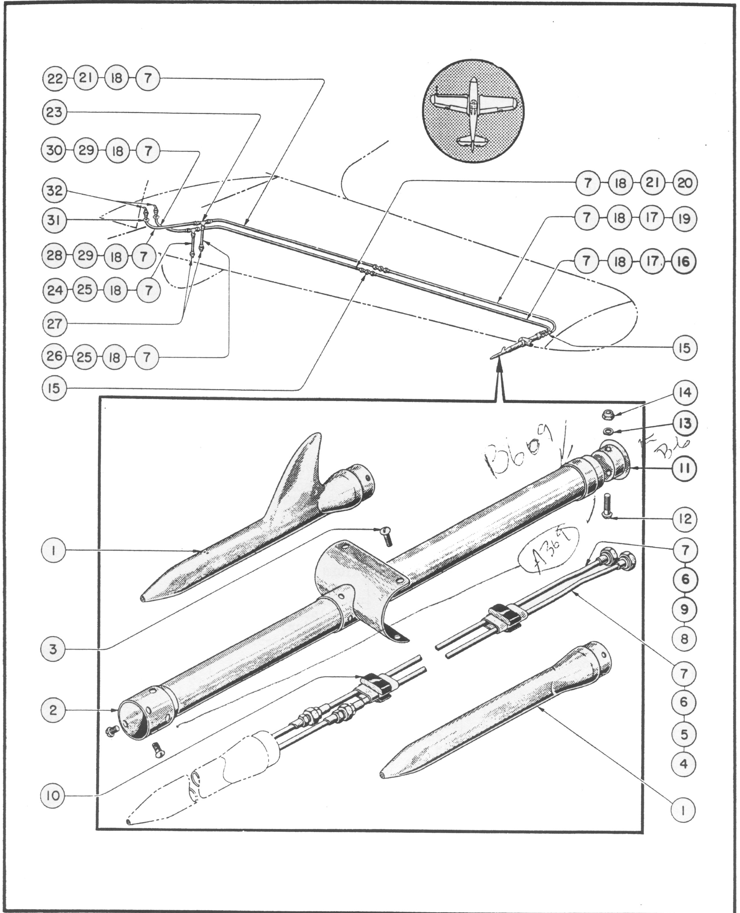
Figure 120—Pitot Static Tube Installation
