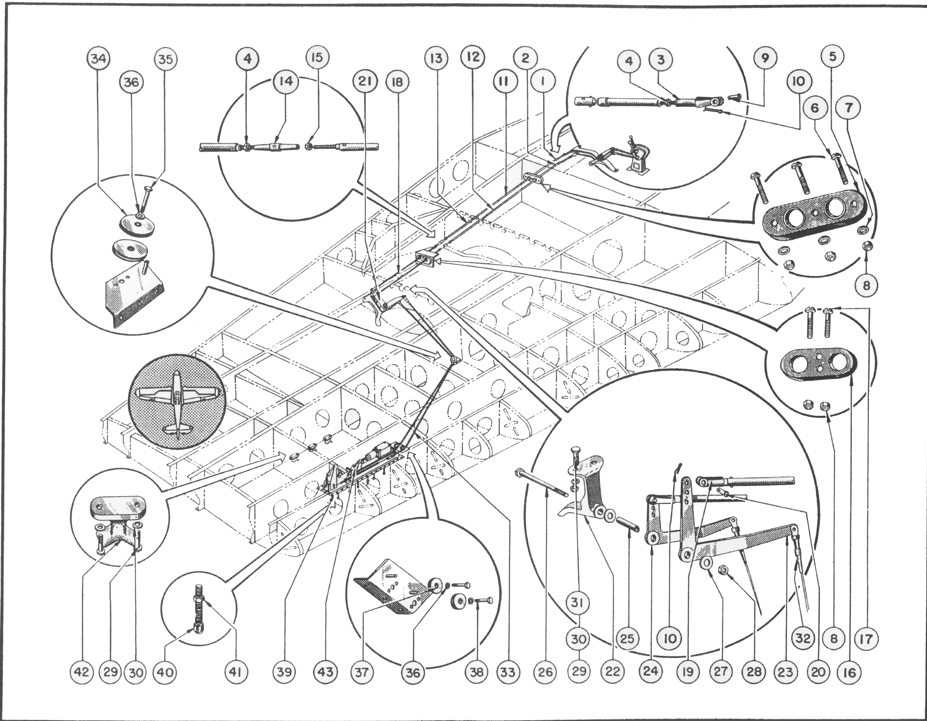
Figure 122—Wing Bomb Installation—Right Wing Panel (A-C)
