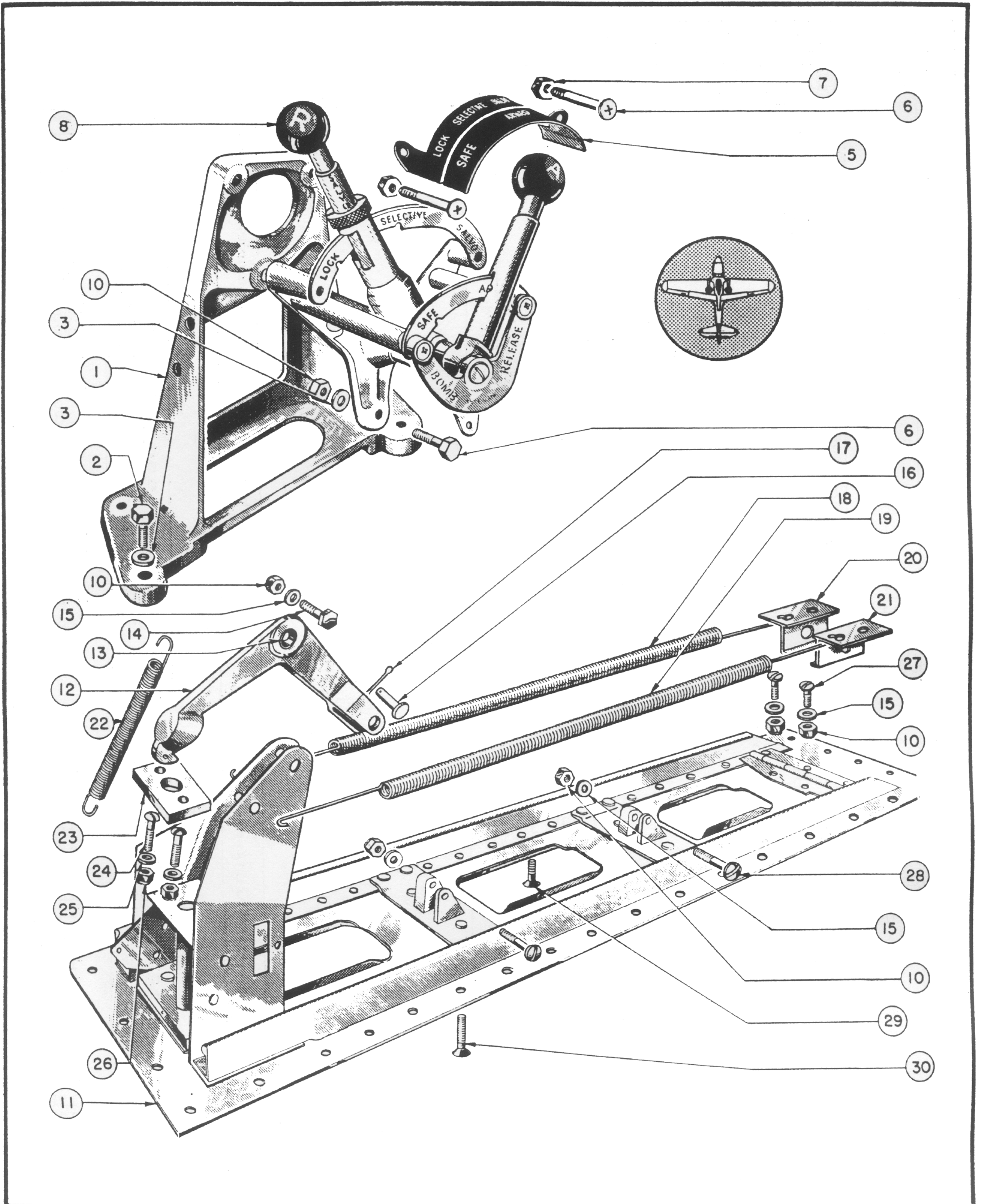
Figure 123—Bomb Control and Bomb Rack Door Assembly
