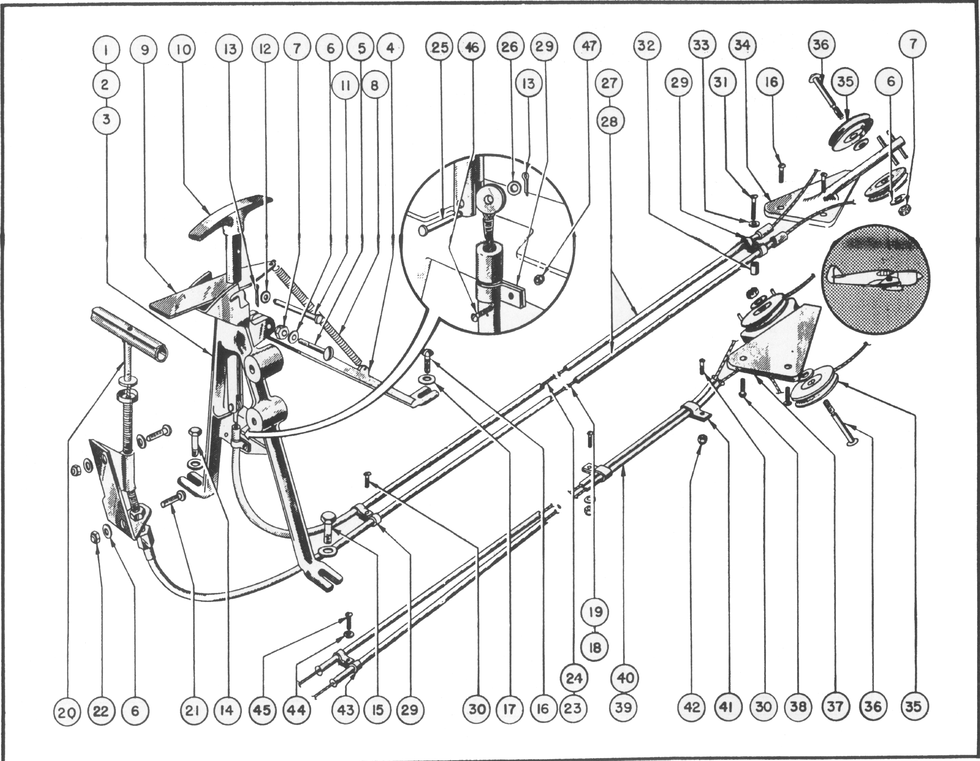
Figure 127—Bomb and Belly Tank Installation
