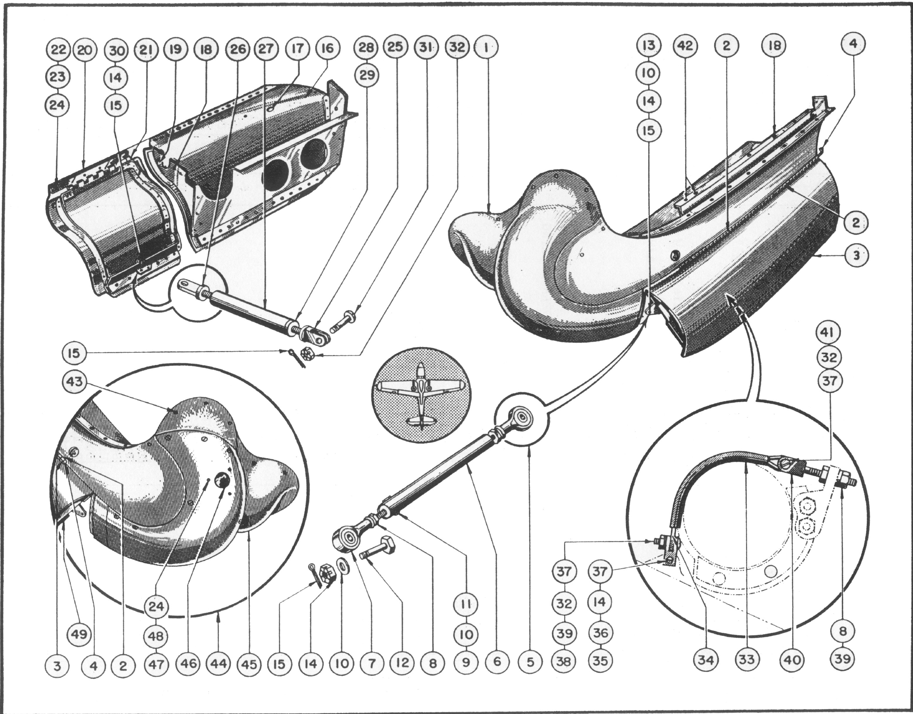
Figure 13—Landing Gear Fairing Assembly
