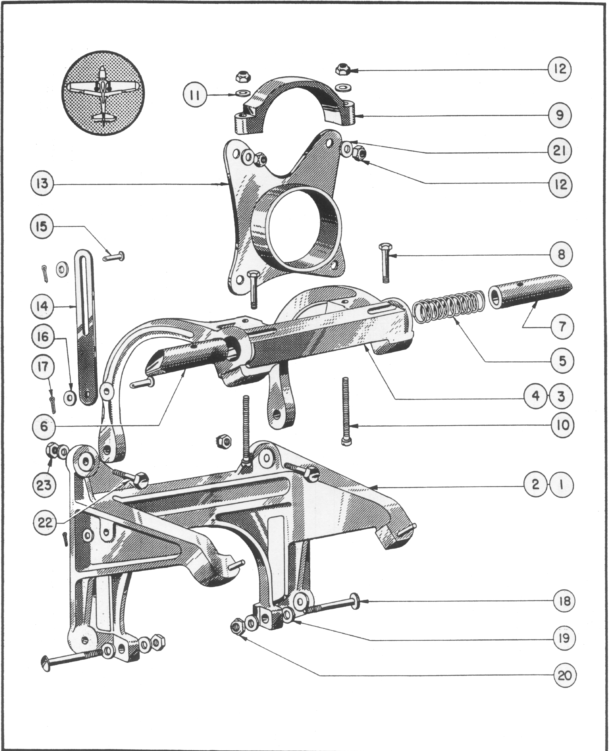
Figure 130—Gun Camera Installation (A-V)
