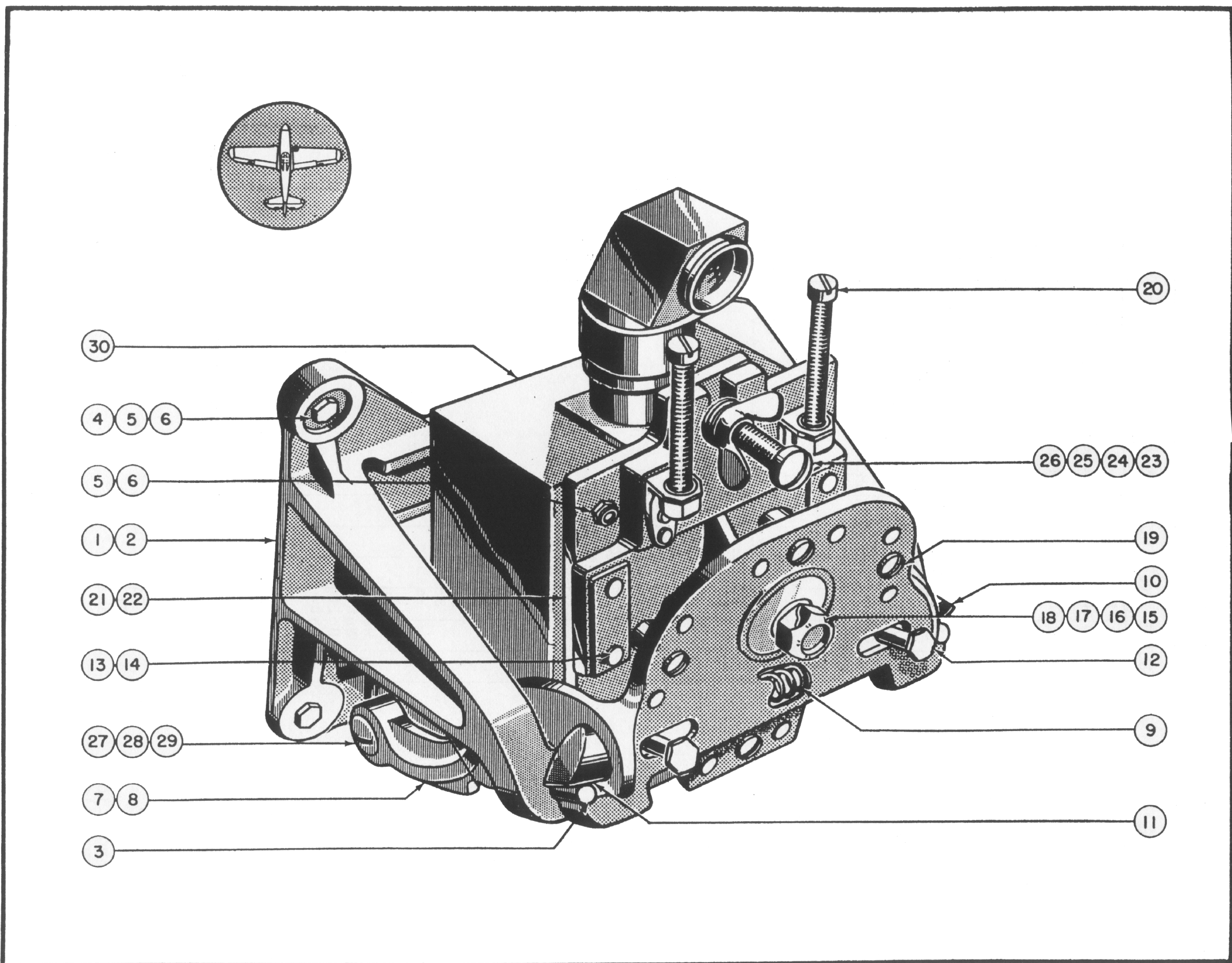
Figure 131—Gun Camera Installation (W)
