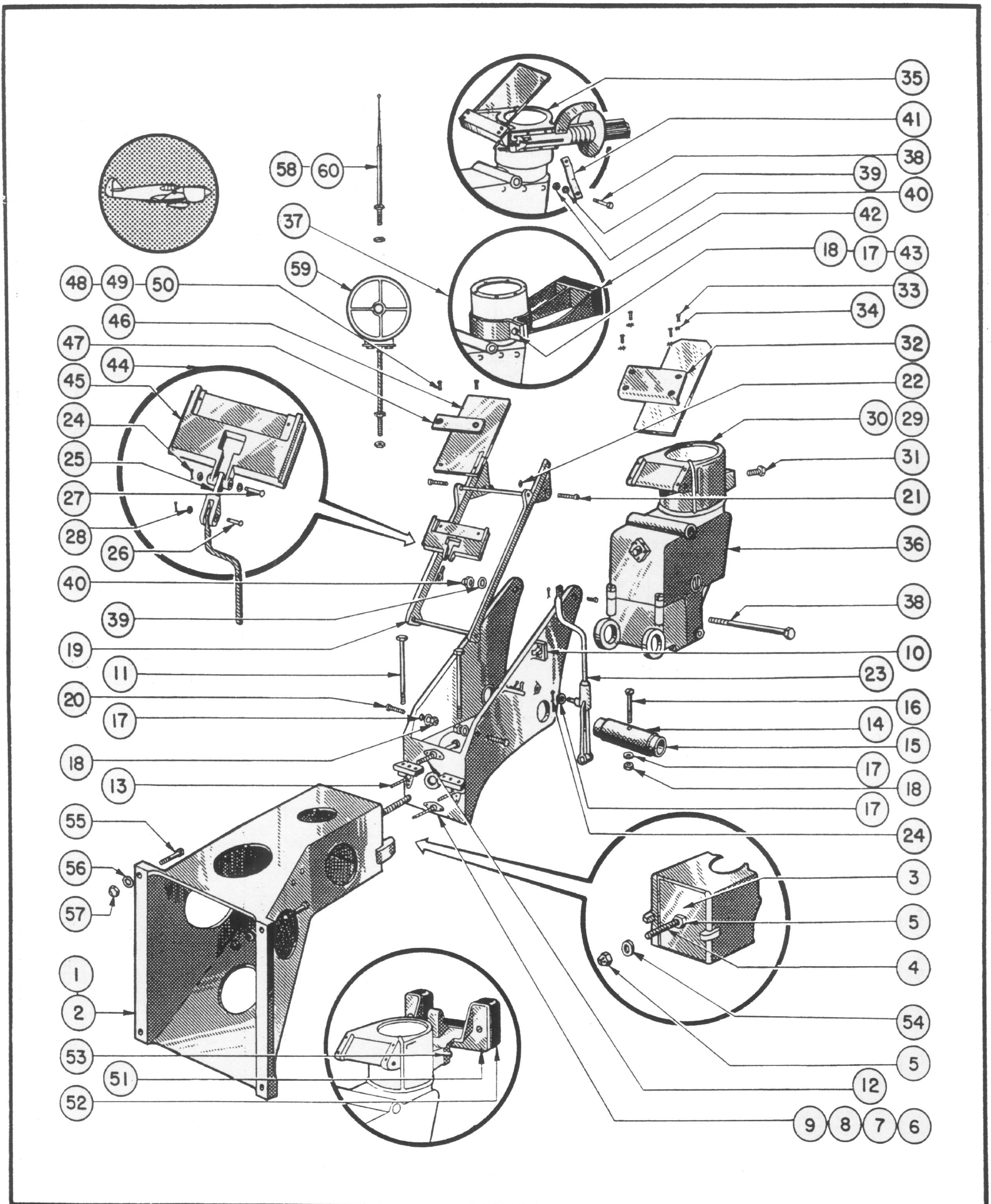
Figure 132—Gun Sight Installation
