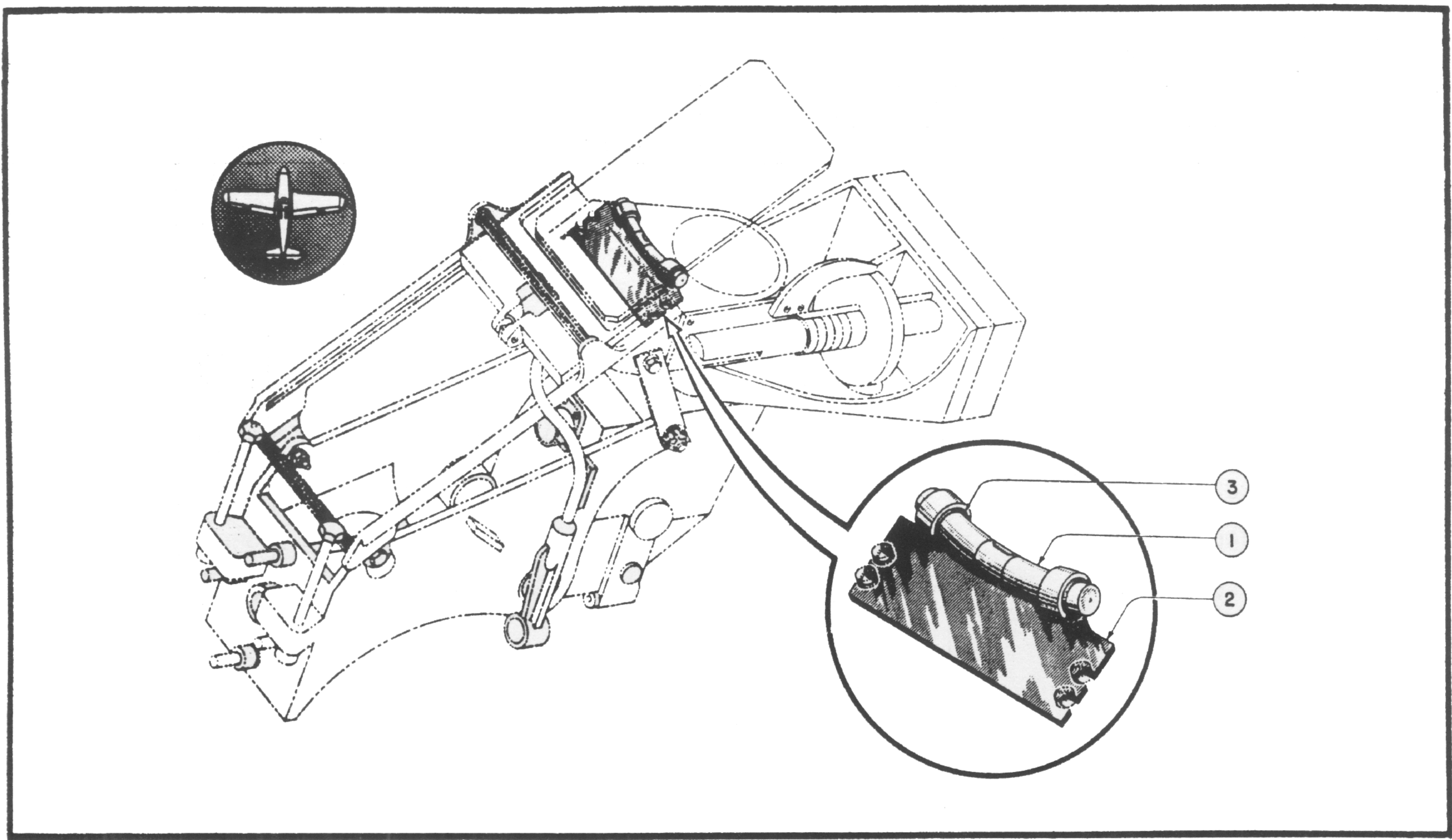
Figure 133—Gun Sight Inclinator Assembly
