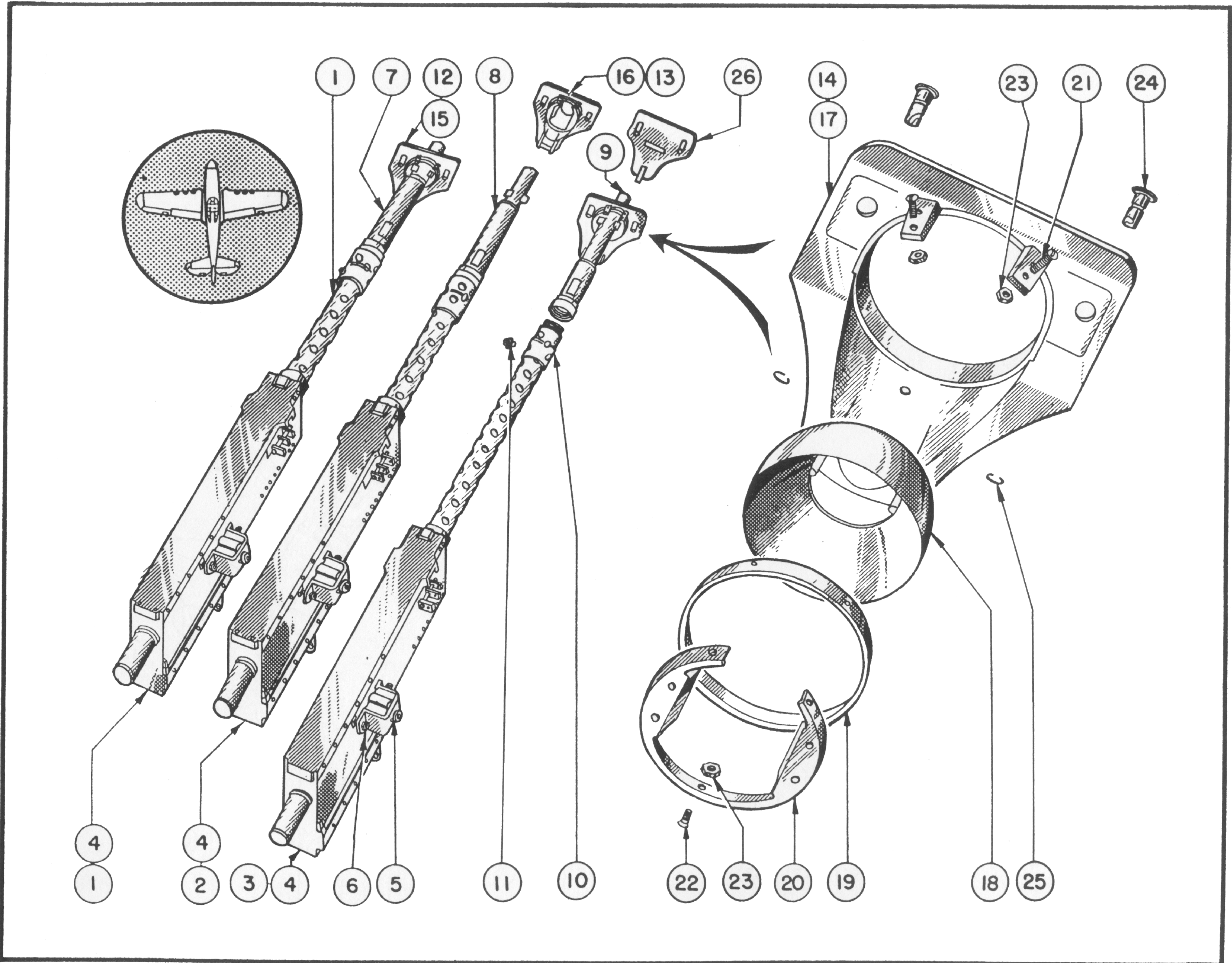
Figure 134—.50 Caliber Wing Gun Installation
