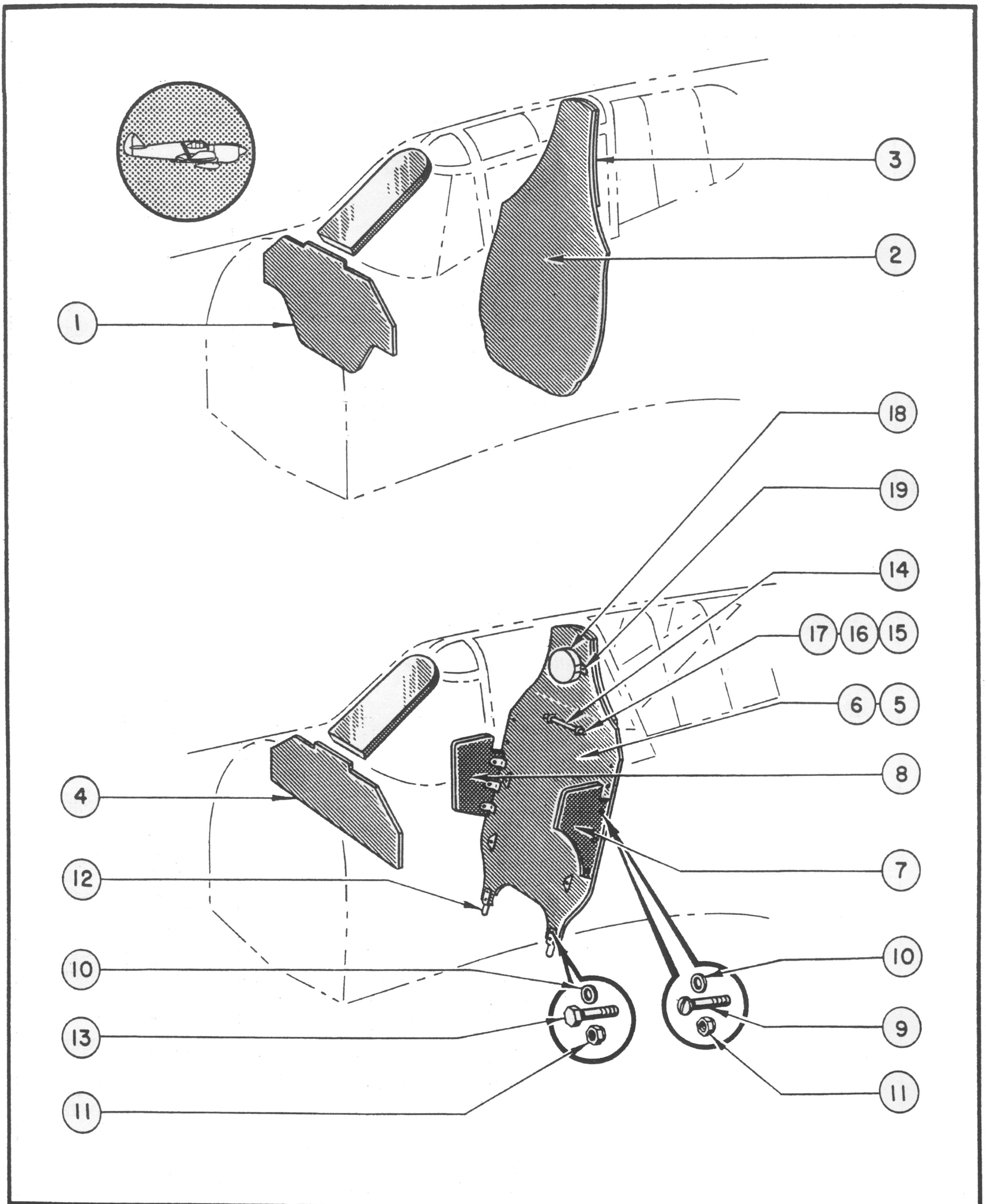
Figure 137—Armor Plate
