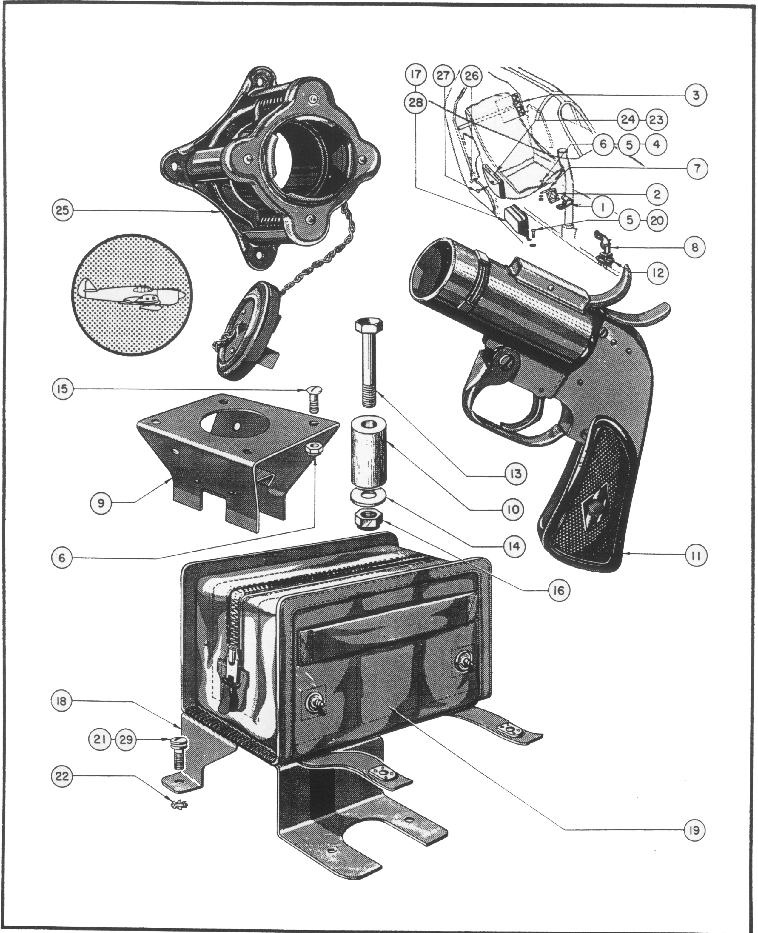
Figure 138—Pyrotechnic Installation
