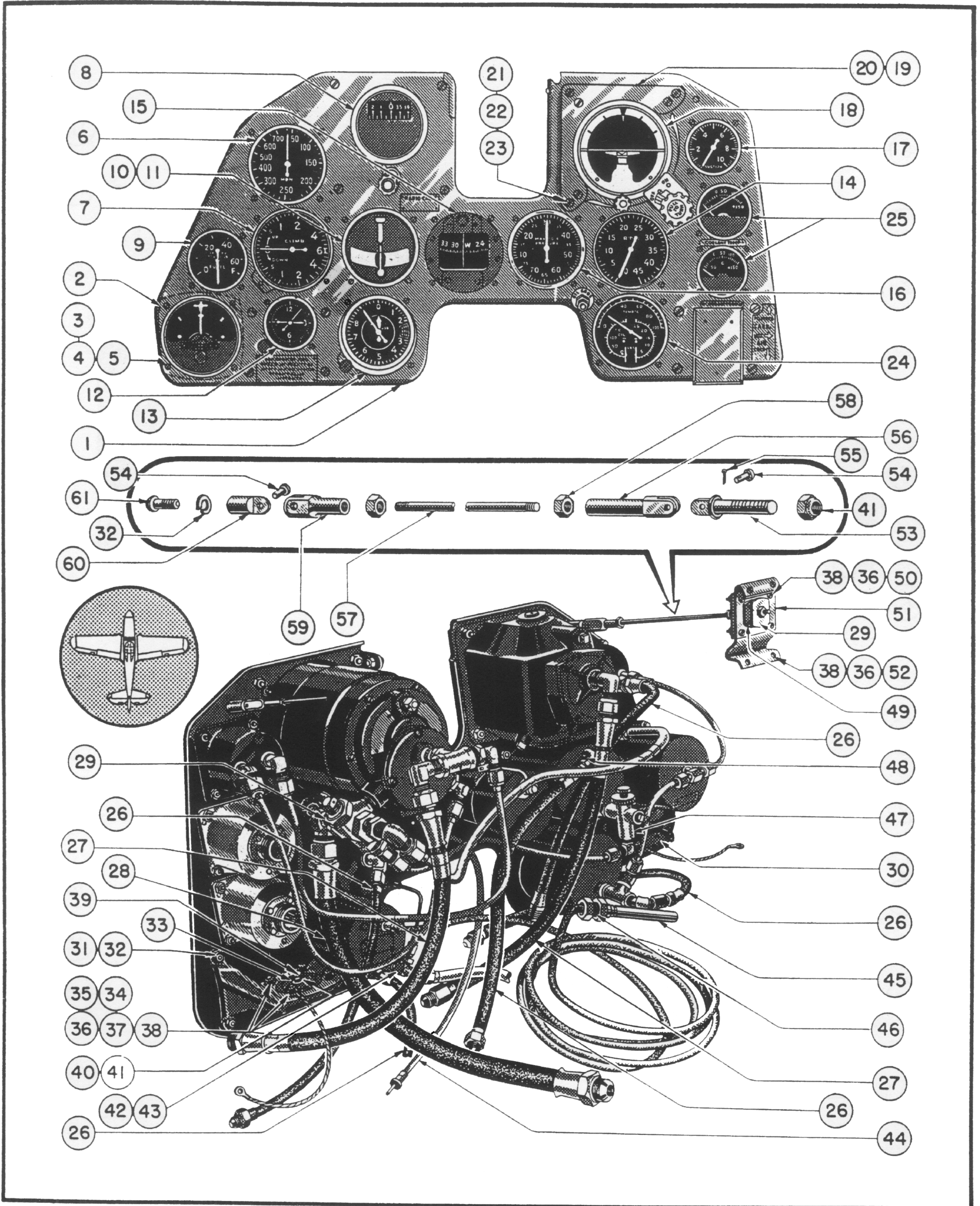
Figure 141—Instrument Installation & Gyro Hook-Up (T-W)
