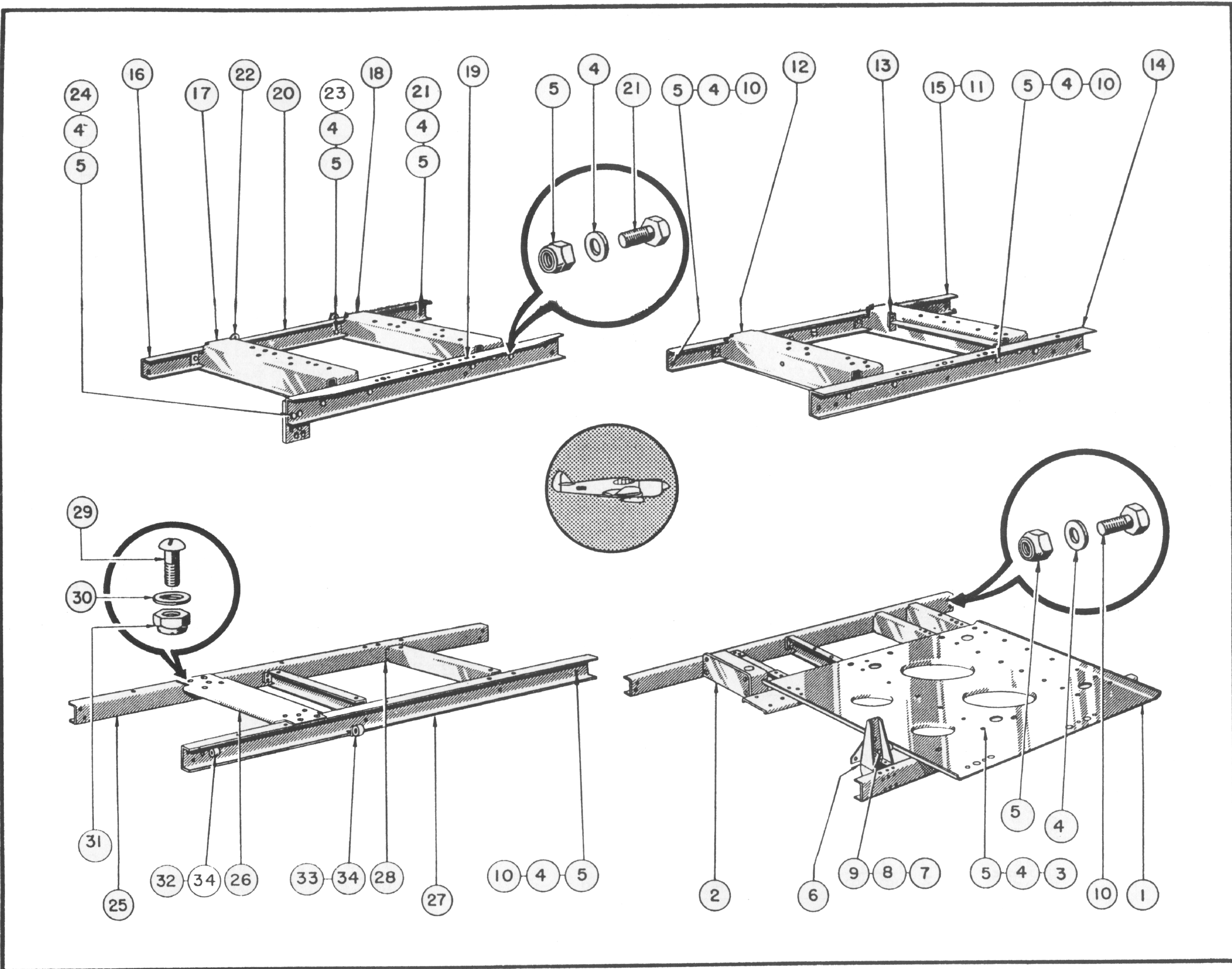
Figure 142—Radio Support Shelf Installation
