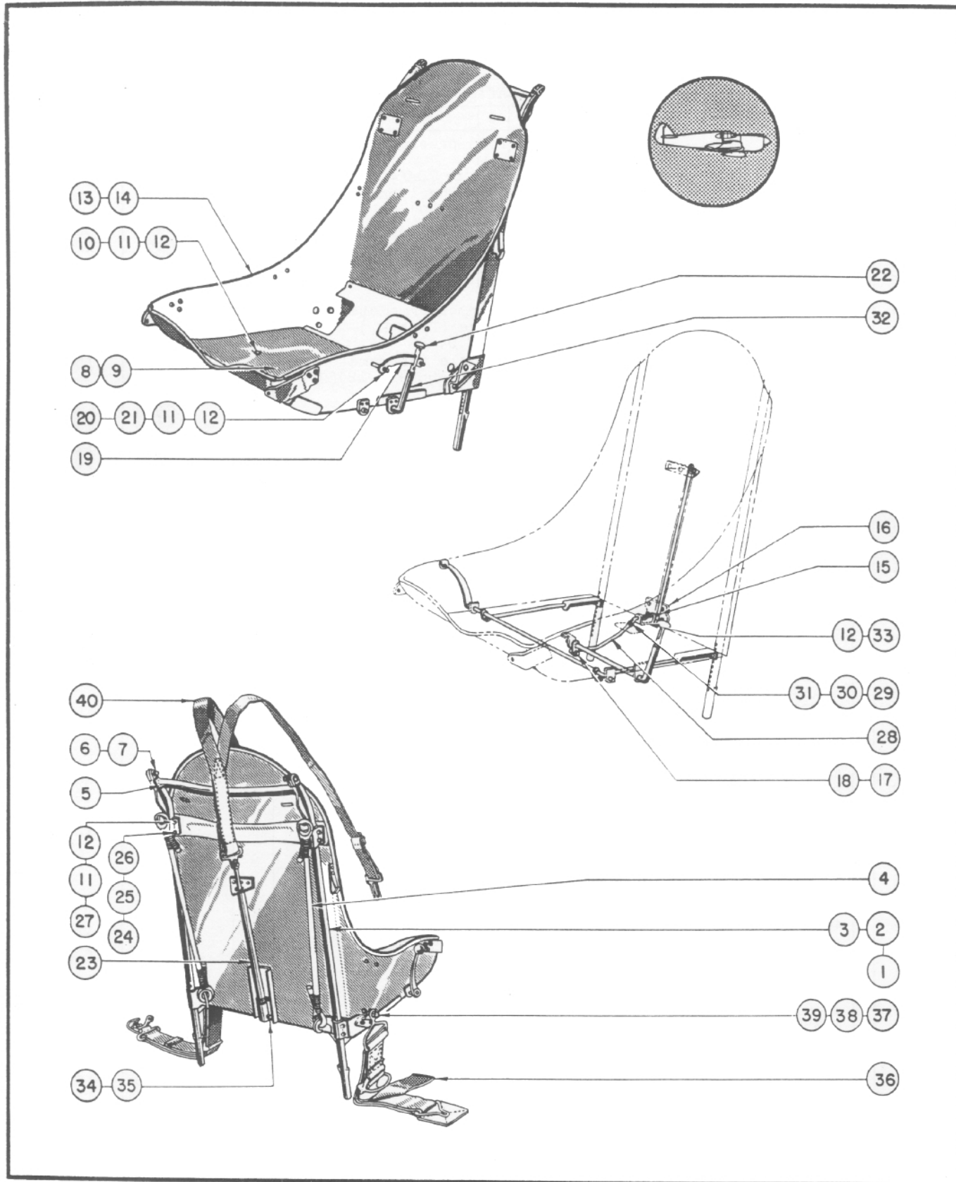
Figure 143—Seat Assembly (A-C)
