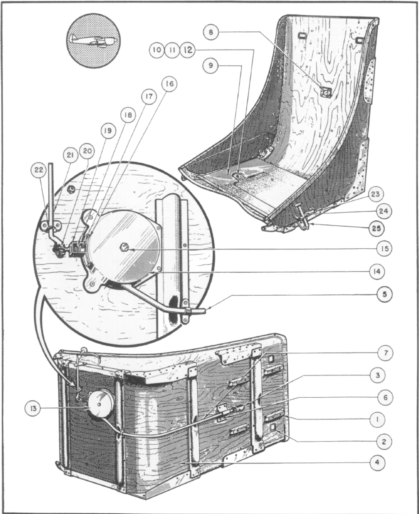
Figure 144—Seat Assembly (D-W)
