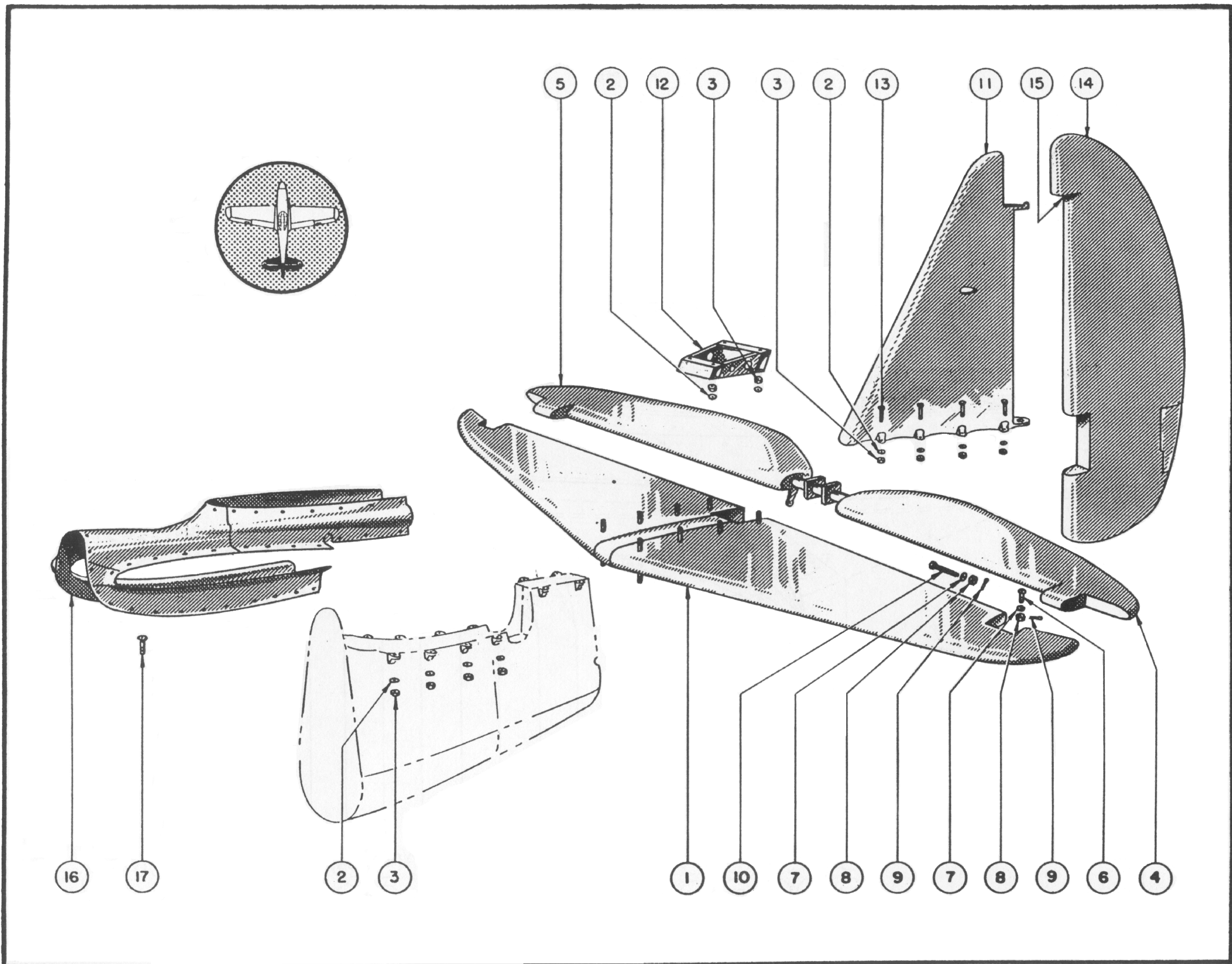
Figure 15—Tail Erection
