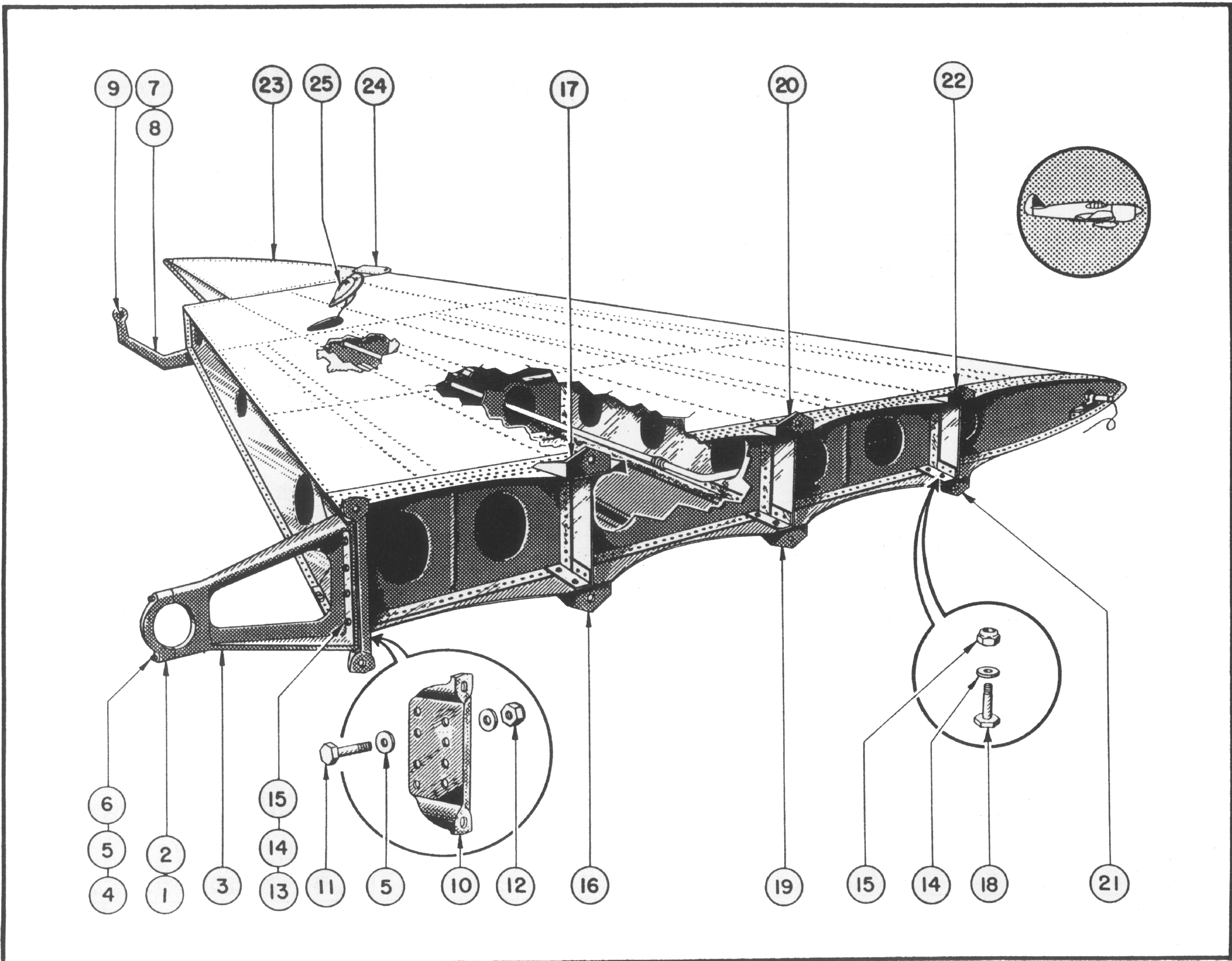
Figure 16—Fin Assembly
