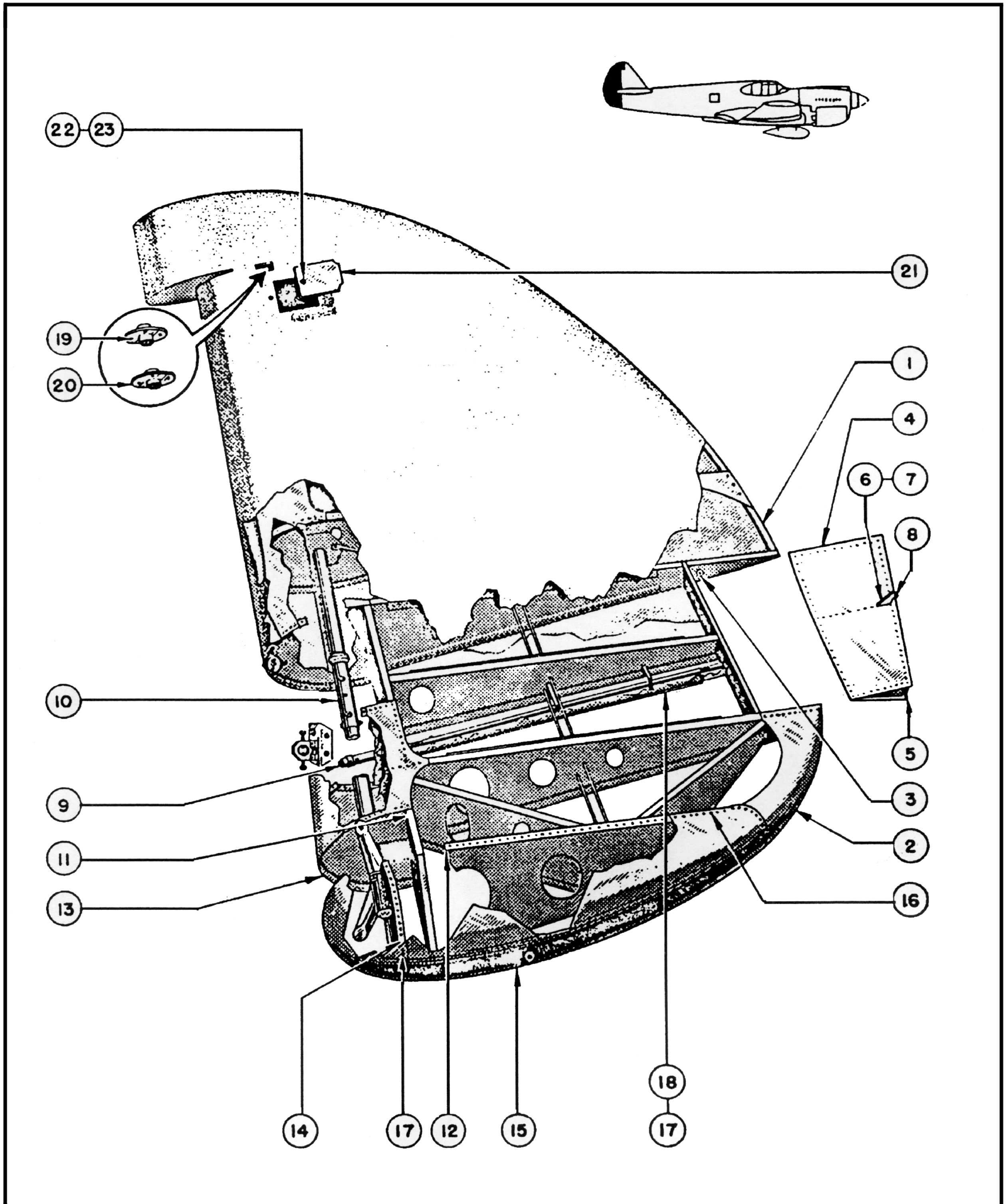
Figure 17 - Rudder
