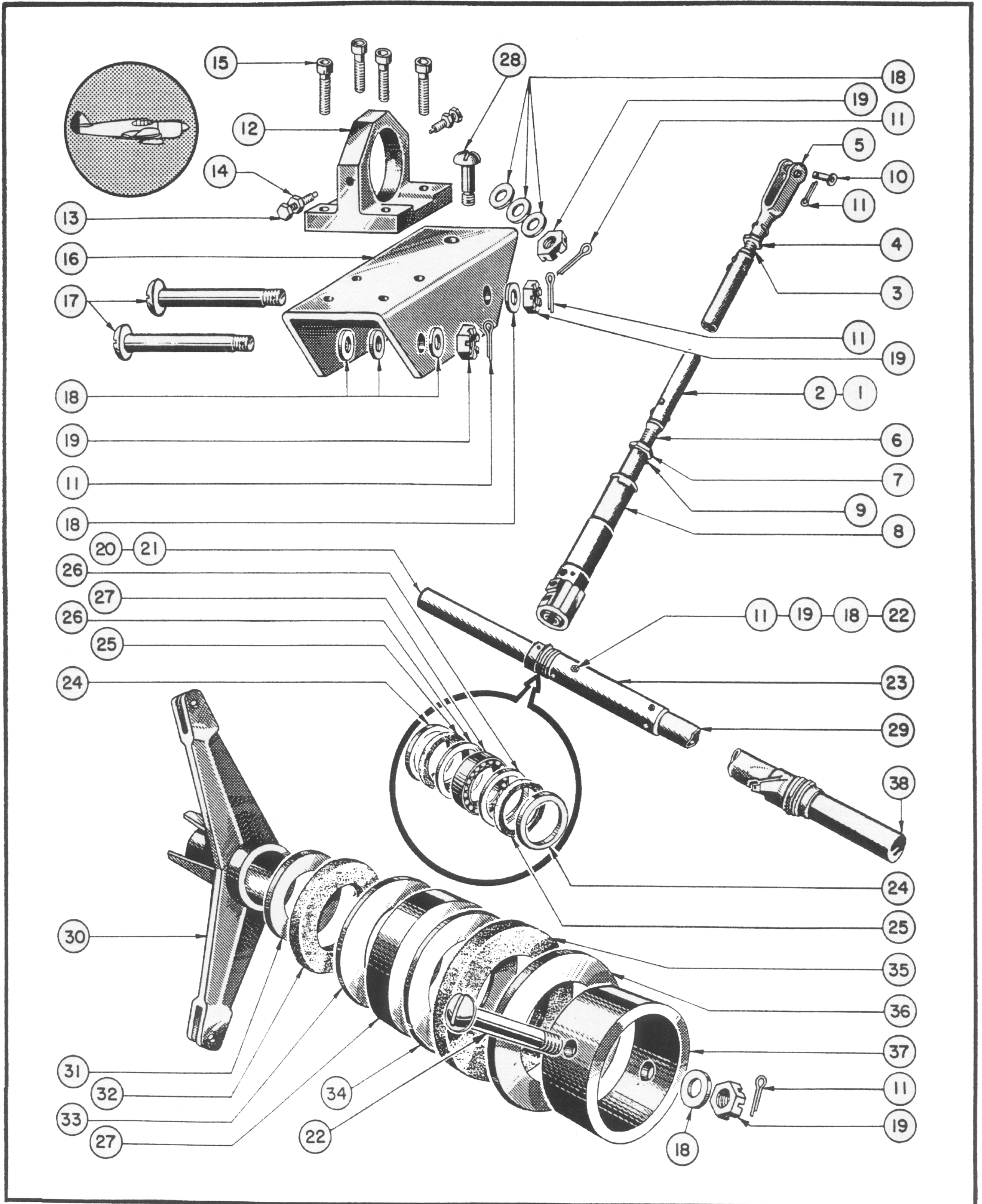
Figure 18—Rudder Torque Tube & Trim Tab Tube
