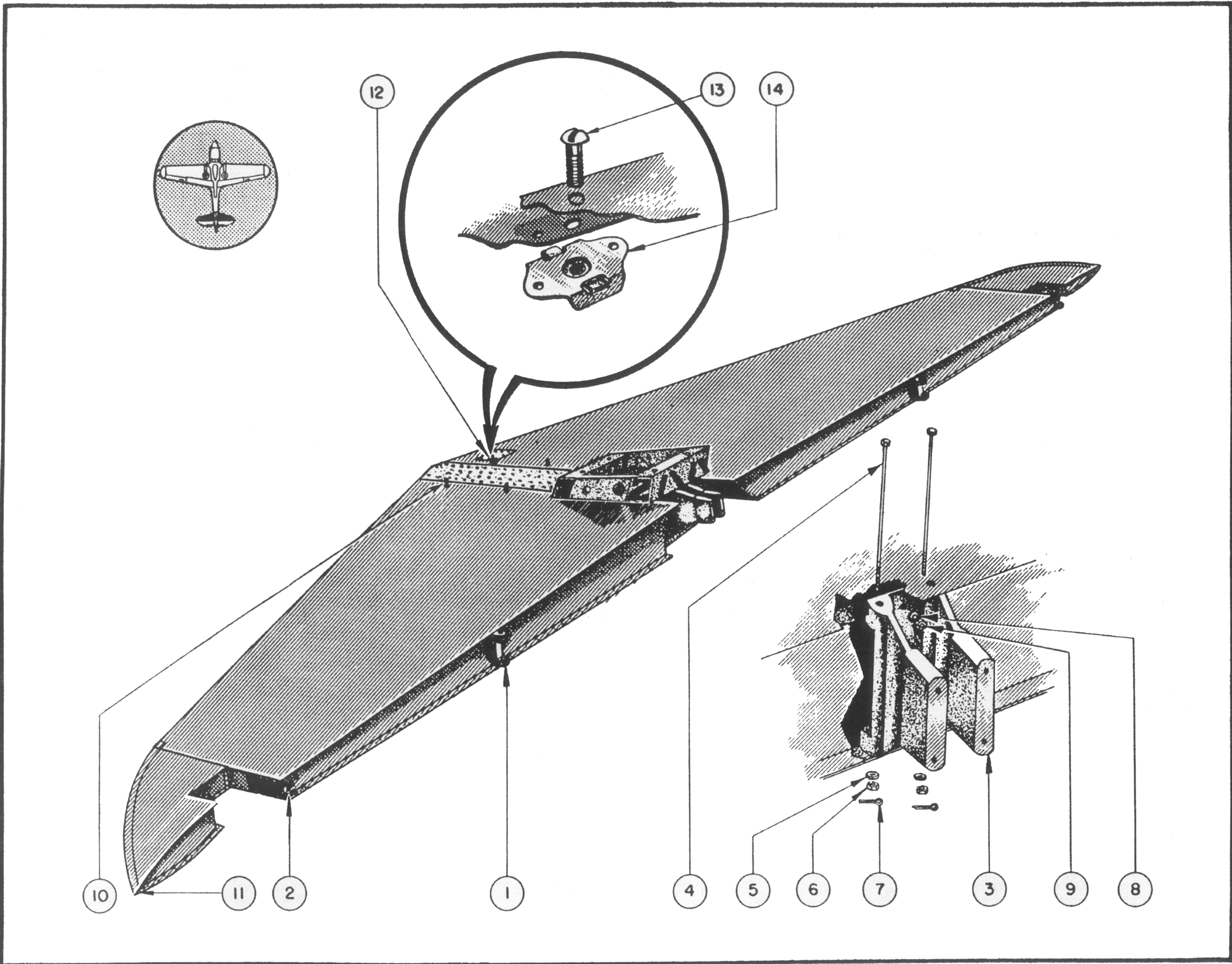
Figure 19—Stabilizer Assembly
