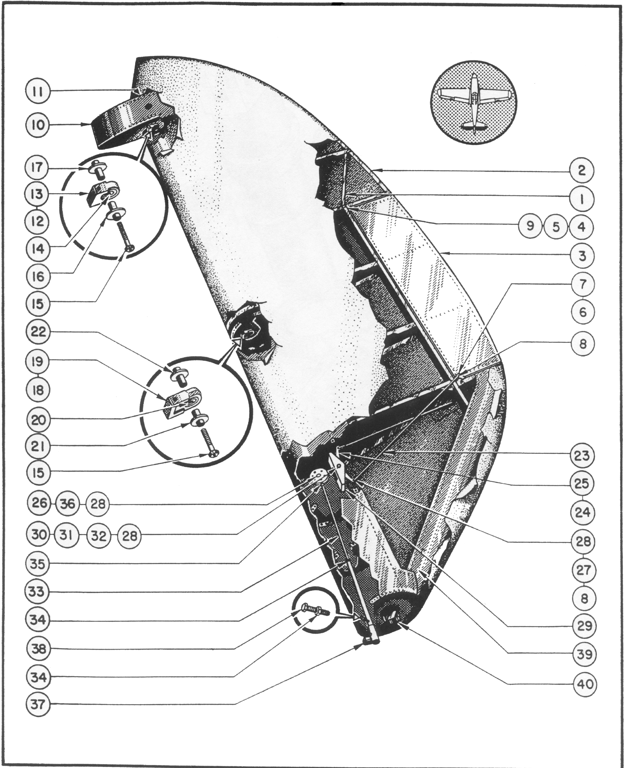
Figure 20—Elevator Assembly
