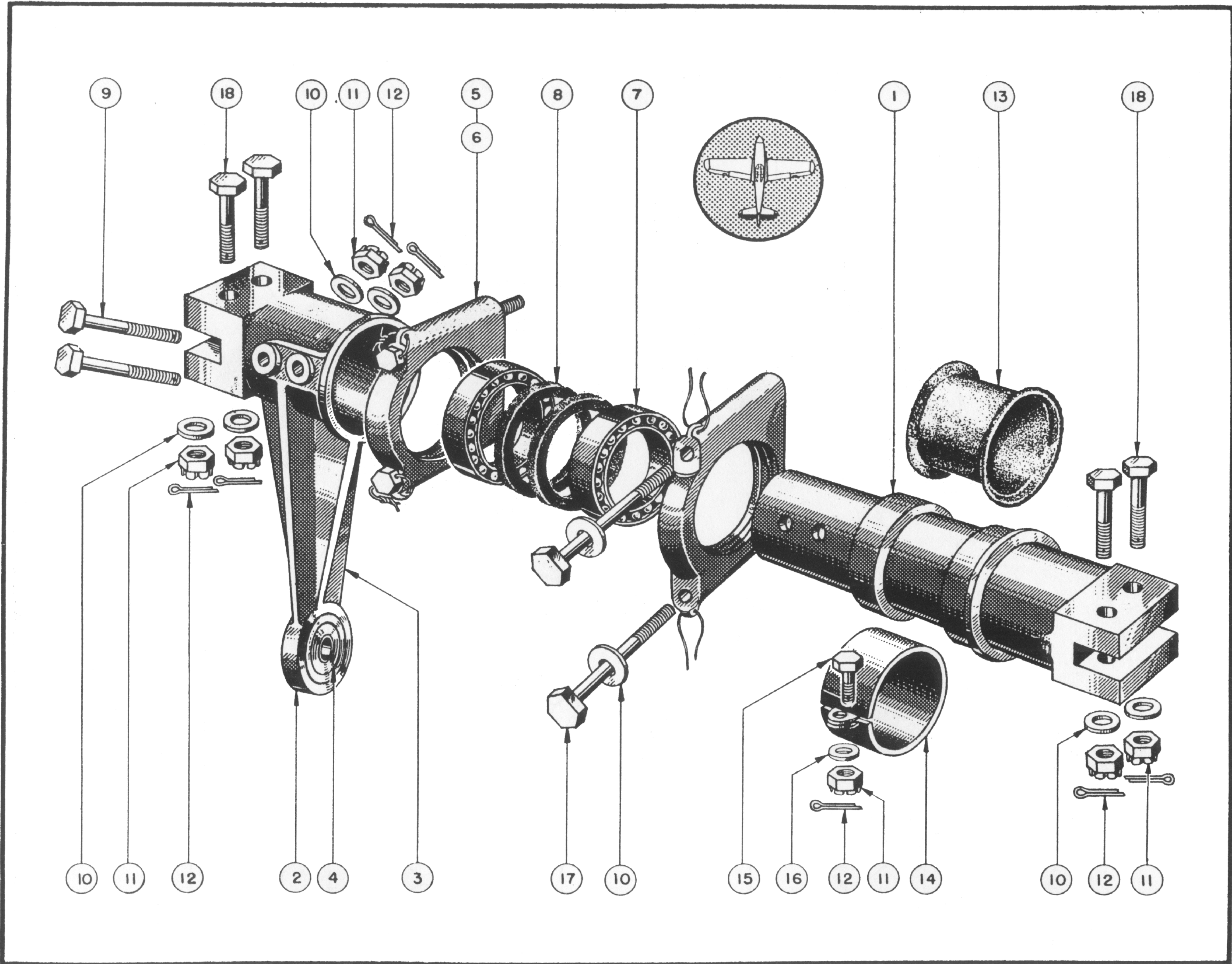
Figure 21—Elevator Bearing Assembly
