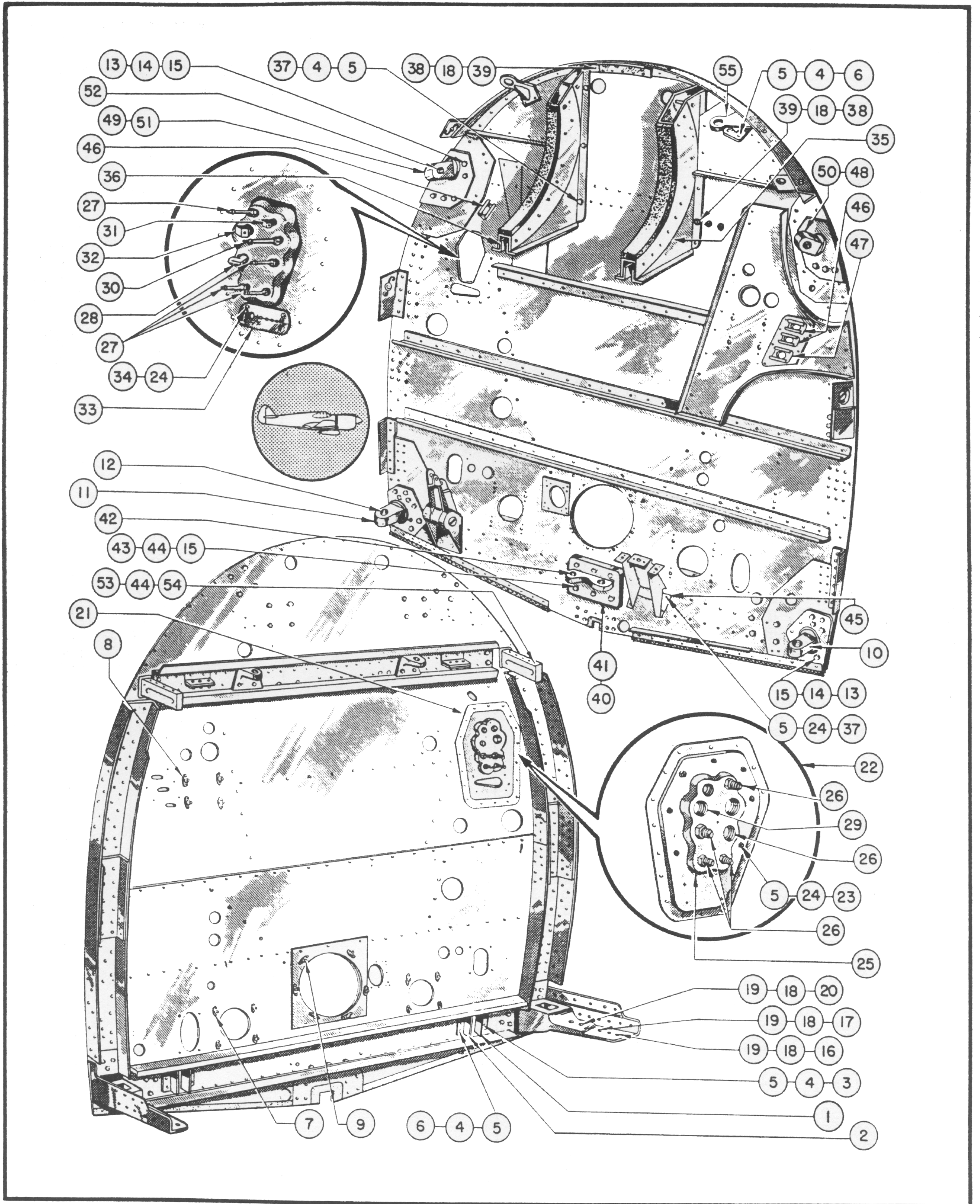
Figure 23—Station Number 1 Firewall Bulkhead (A-B)
