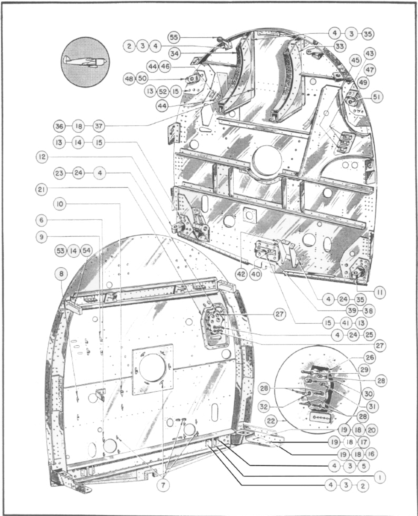
Figure 24—Station Number 1 Firewall Bulkhead (C-V)
