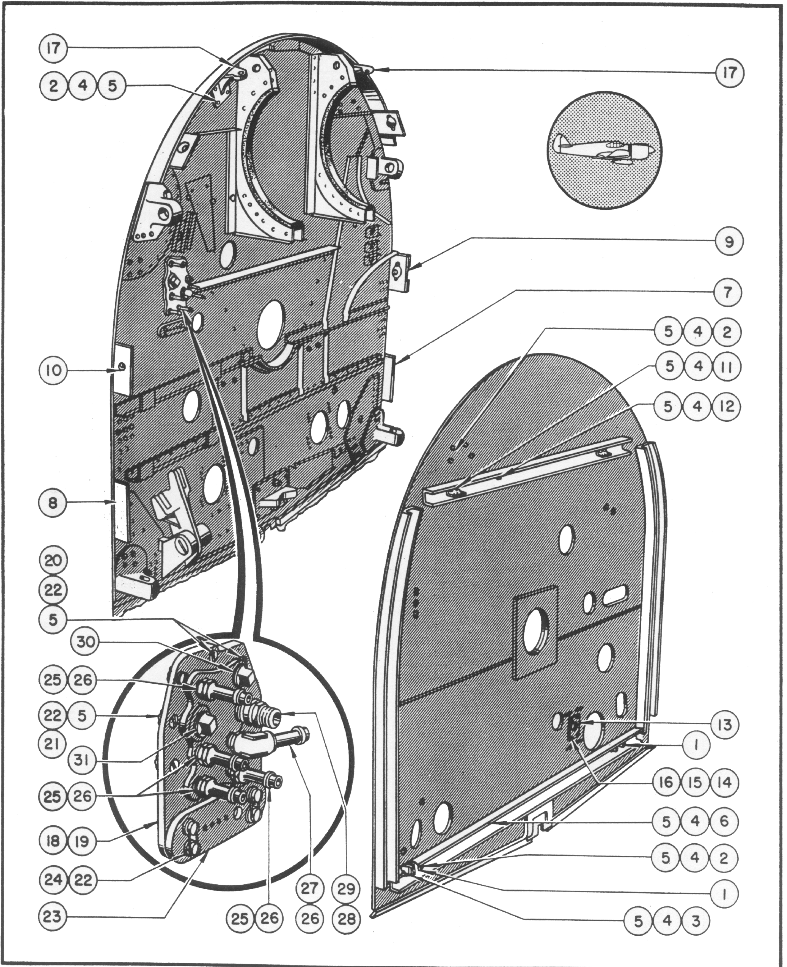
Figure 25—Station Number 1 Firewall Bulkhead (W)
