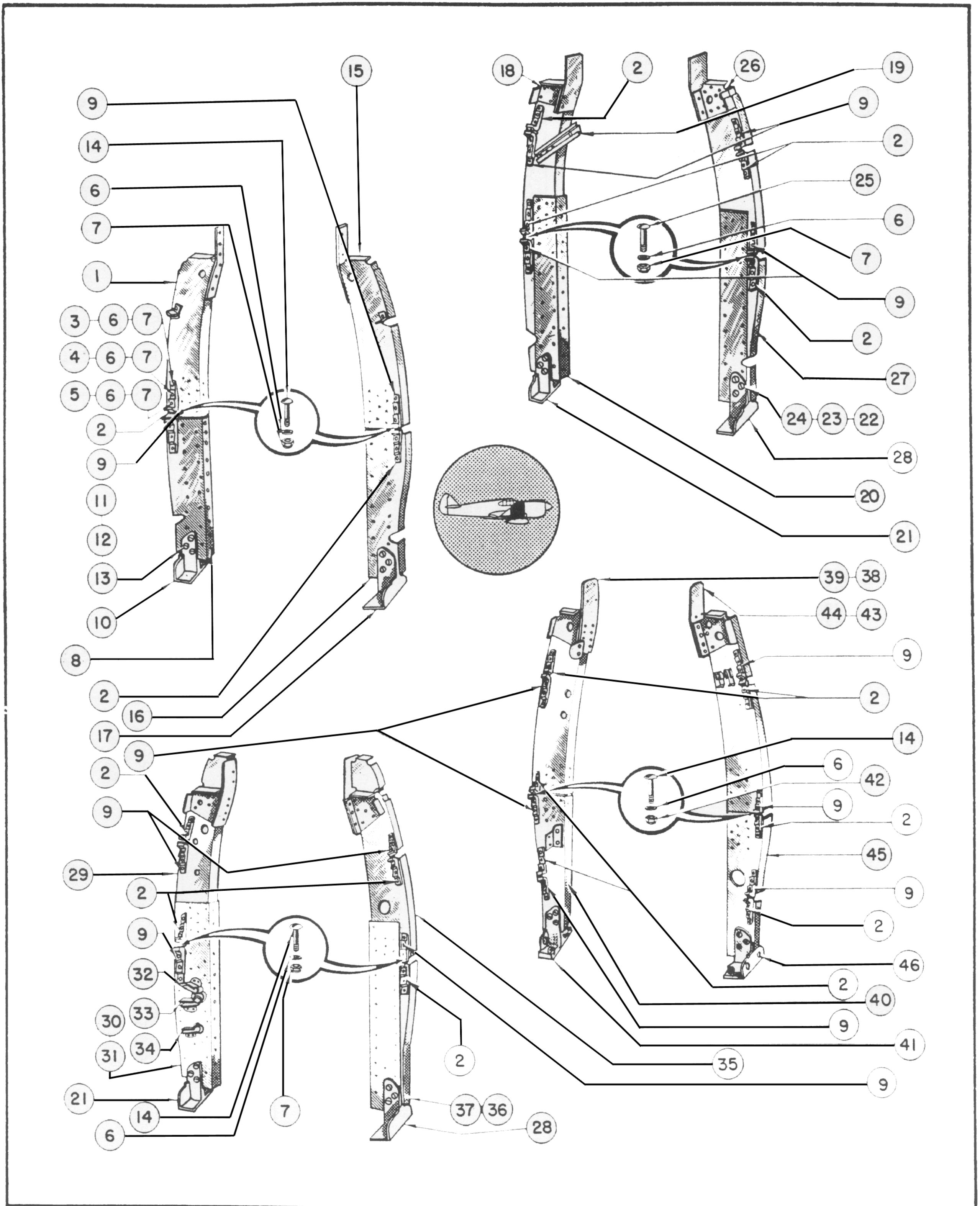
Figure 26—Bulkhead Assemblies Stations 1A, 2, 3, and 4
