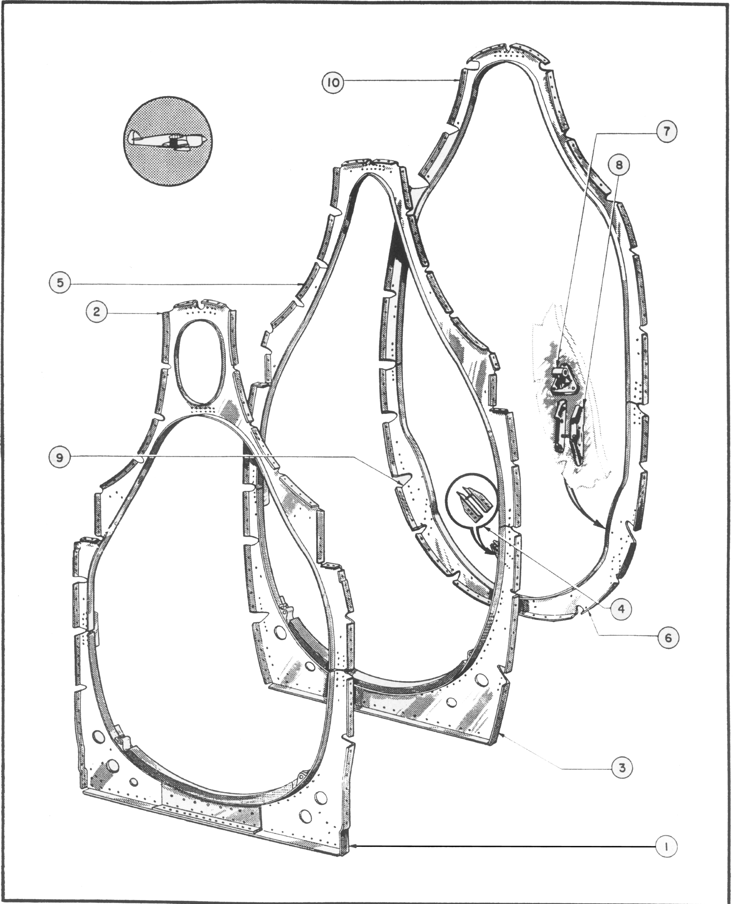
Figure 27—Bulkhead Assemblies Stations 6, 7, and 8 (A-C)
