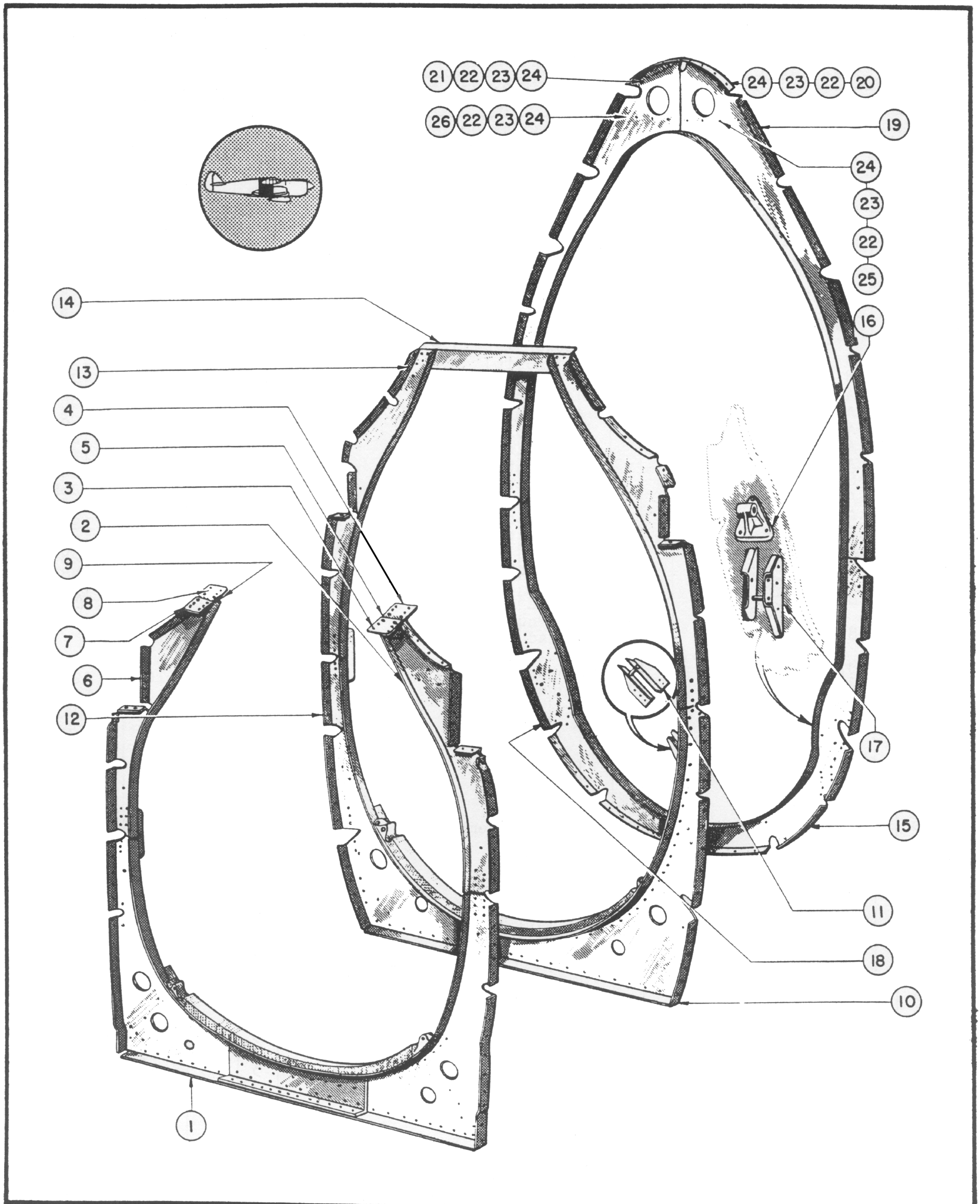
Figure 28—Bulkhead Assemblies Stations 6, 7, and 8 ( D-W)
